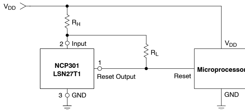
Figure 30. Microprocessor Reset Circuit with Additional Hysteresis
