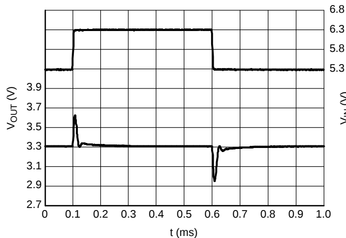
Figure 31. Line Transients, 3.3 V Version, t_R = t_F = 5 \mu s , I_{OUT} = 30 mA
