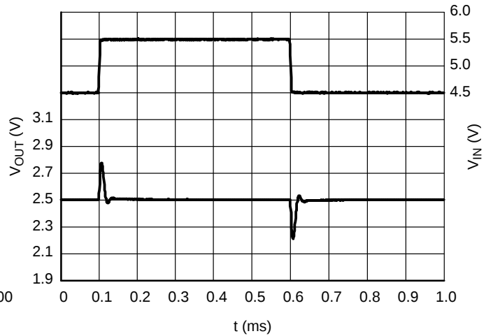
Figure 30. Line Transients, 2.5 V Version, t_R = t_F = 5 \mu s , I_{OUT} = 30 mA
