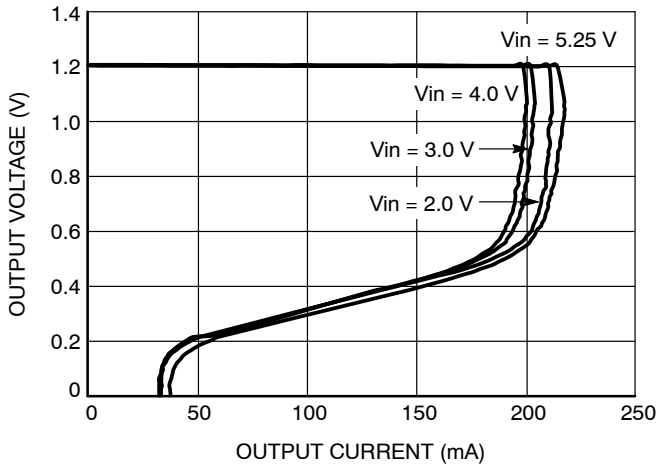
Figure 3. Output Voltage vs. Output Current NCP4688xx12
