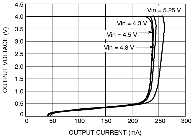
Figure 5. Output Voltage vs. Output Current NCP4688xx40
