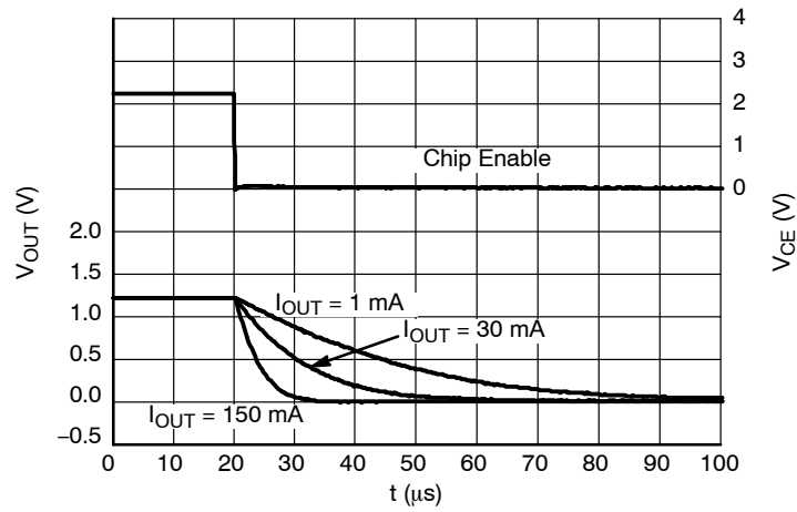
Figure 39. Shutdown, 1.2 V Version D, V_{IN} = 2.2 V
