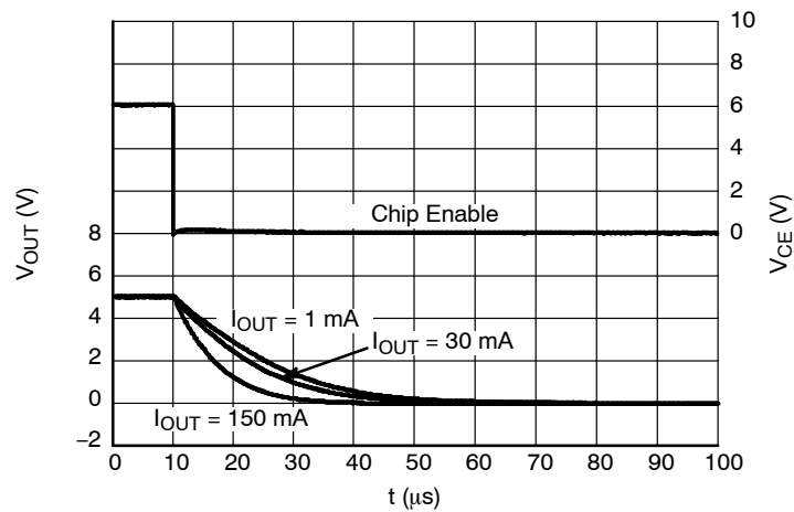
Figure 41. Shutdown, 5.0 V version D, V_{IN} = 6.0 V
