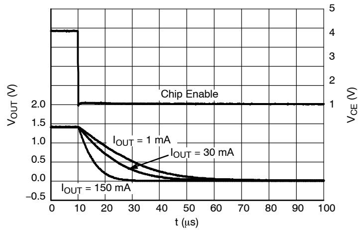
Figure 40. Shutdown, 2.8 V Version D, V_{IN} = 3.8 V
