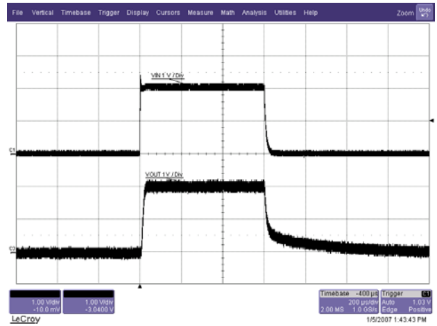
Figure 11. Turn-on Response
