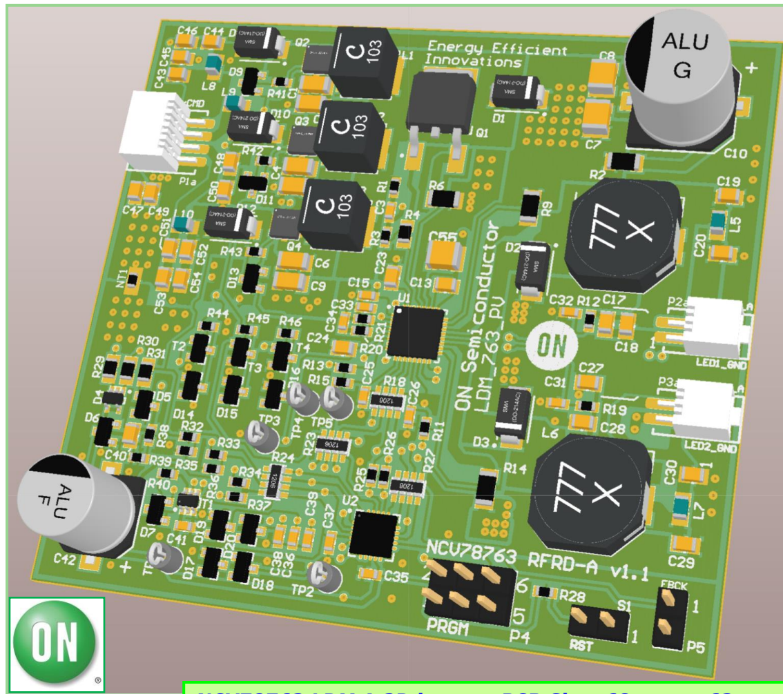
NCV78763 LDM A 3D image - PCB Size: 68mm xx 63mm
