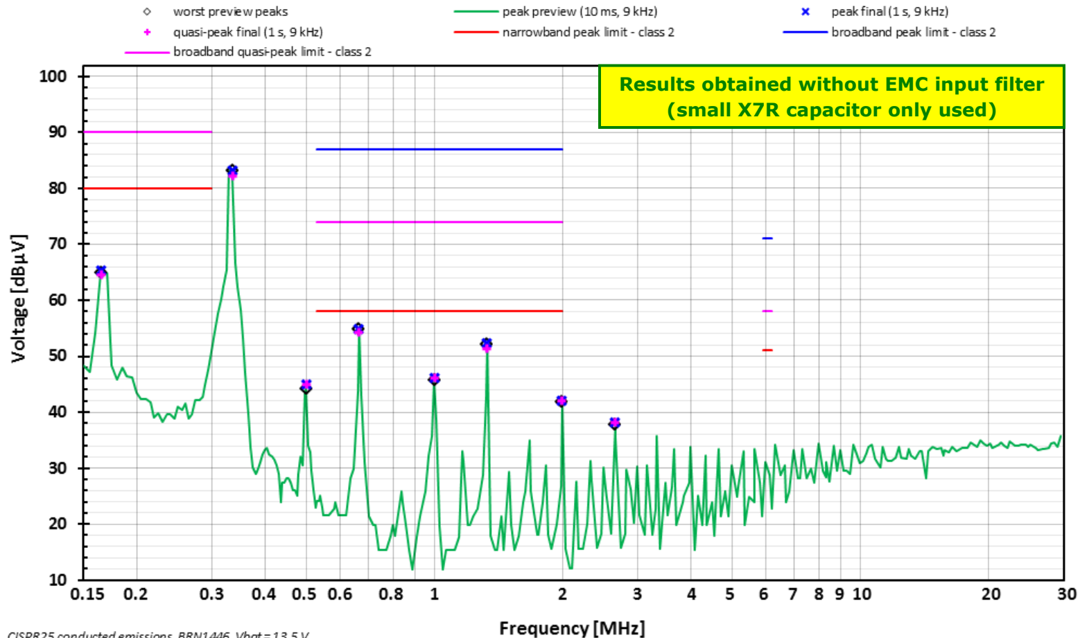
NCV78763 reference design board RFRD-A v1.1 (DRL & TI inputs powered)
