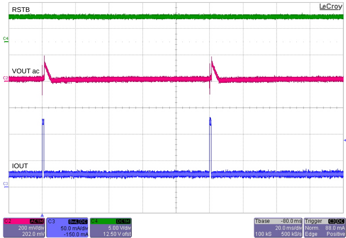
Figure 31. V_{IN} = 13\text{ V} , V_{OUT} = 5\text{ V} , 20 mA to 120 mA Load Transient – with Mode Transition
