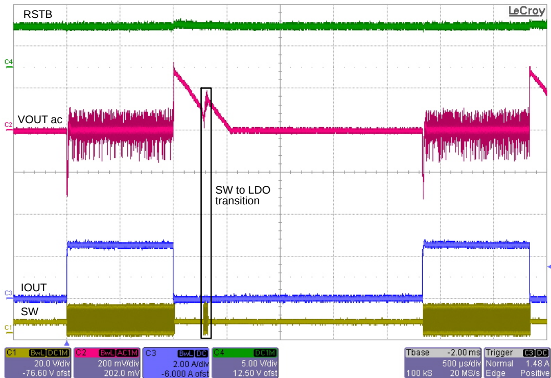
Figure 29. V_{IN} = 13 V, V_{OUT} = 5 V, 20 mA to 2.5 A at 1 A/ \mu s – with Mode Transition
