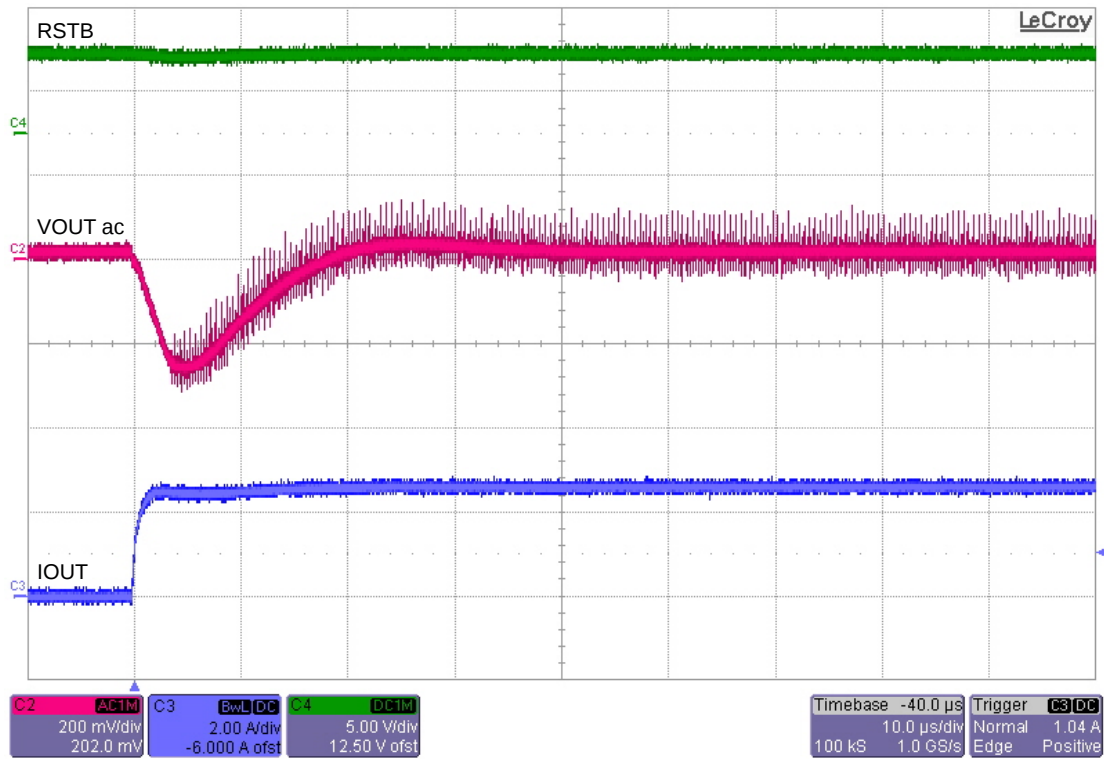
Figure 30. Detail of the 20 mA to 2.5 A Transition at V_{IN} = 13\text{ V} and V_{OUT} = 5\text{ V}
