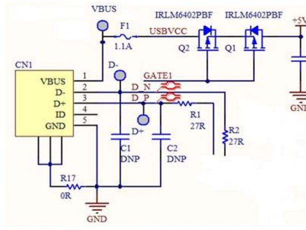
Figure 3 - USB Power Supply
