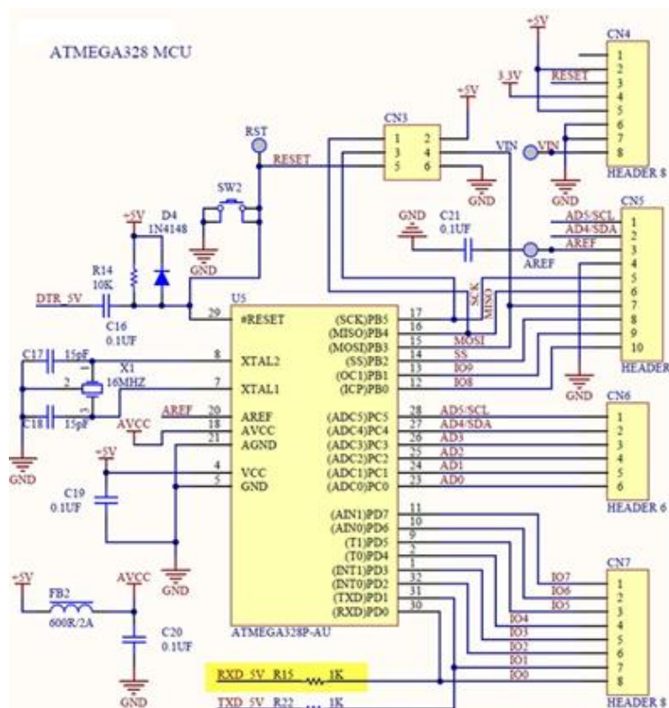
Figure 4 - Atmega328P Micro-controller
