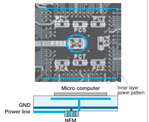
With chip 3-terminal capacitor (NFM) 1 \mu Fx1
