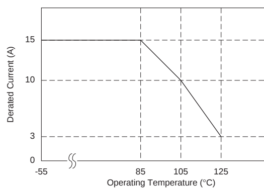
Derating
