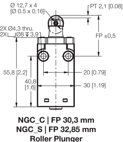
Figure 9. Roller Plunger C & S Dimensions
