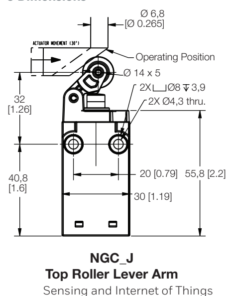
Figure 16. Top Roller Lever Arm J Dimensions
