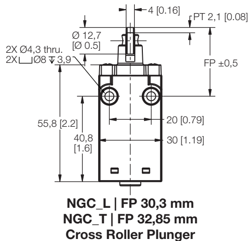
Figure 10. Cross Roller Plunger L & T Dimensions
