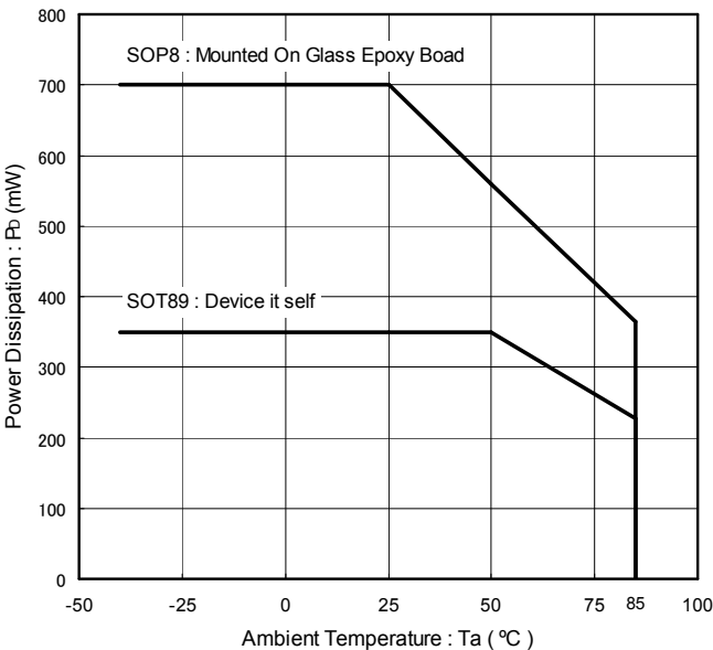
Power Dissipation vs. Ambient Temperature ( T opr = - 40°C ~ + 85°C, T j = ~ +150°C )
