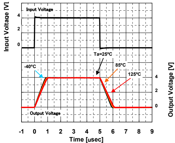
Pulse Response
