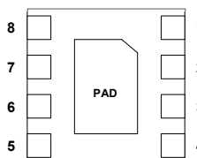
NJU77903KW2 PIN CONFIGURATION
