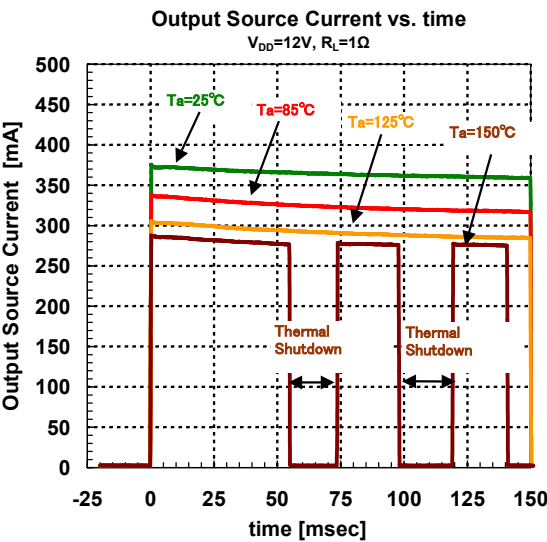
Fig3.3 Output Source Current Limit vs. Time
