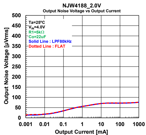
V_{OUT}=2.0V Setting ( R1=5k\Omega , C_o=10\mu F / C_o=22\mu F )
