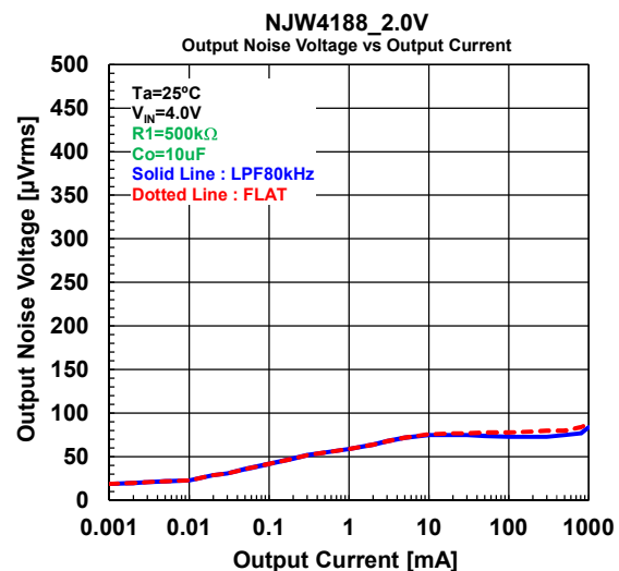
V_{OUT}=2.0V Setting ( R1=50k\Omega / 500k\Omega , C_o=10\mu F )
