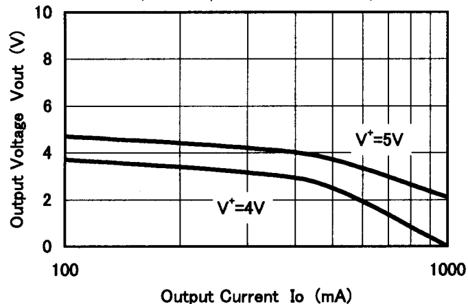
Output Voltage vs. Output Current ( T_a=25^\circ\text{C} , Pulse Measurement)
