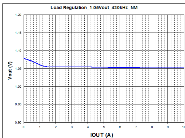
Frequency = 430 kHz
