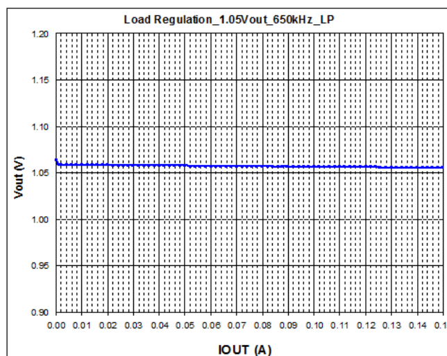
Frequency = 630 kHz
