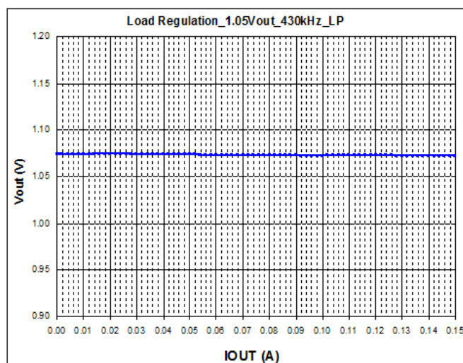
Frequency = 430 kHz
