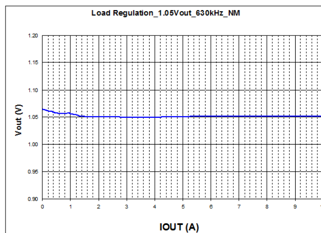
Frequency = 630 kHz
