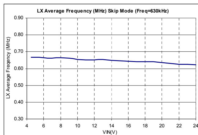
Frequency = 630 kHz
