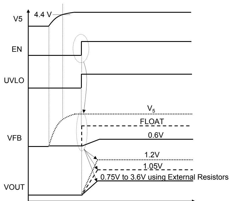
Figure : Timing chart of output voltage setting
