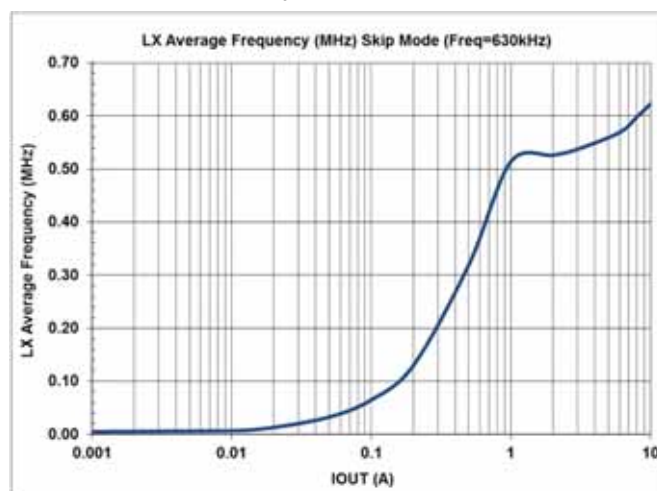
Frequency = 630 kHz
