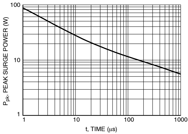
Figure 6. Pulse Width
