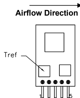
Figure 54. T_{ref} Temperature measurement location.
