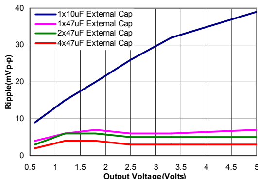
Figure 47. Output ripple voltage for various output voltages with external 1x10 µF, 1x47 µF, 2x47 µF or 4x47 µF ceramic capacitors at the output (3A load). Input voltage is 12V.
