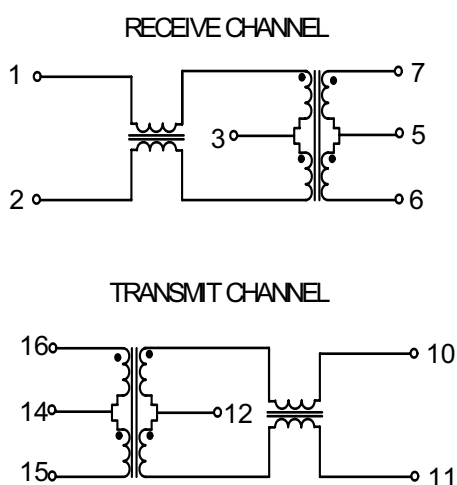
CIRCUIT 7
