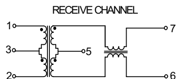
CIRCUIT 6
