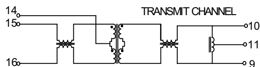
CIRCUIT 4
