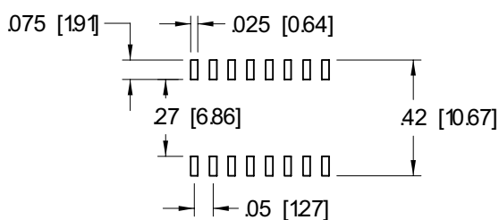
PACKAGE 3
