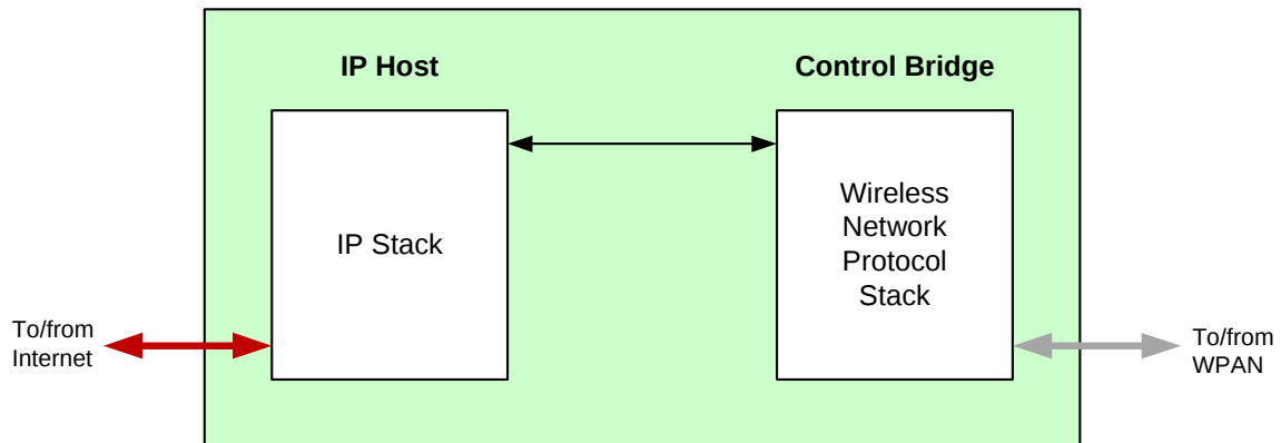
Figure 8: Basic Architecture of an IoT Gateway
