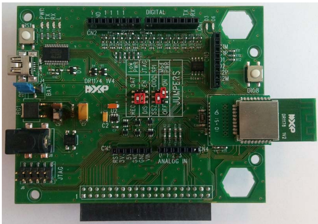
Figure 16: Carrier Board (with a JN516x Module)
