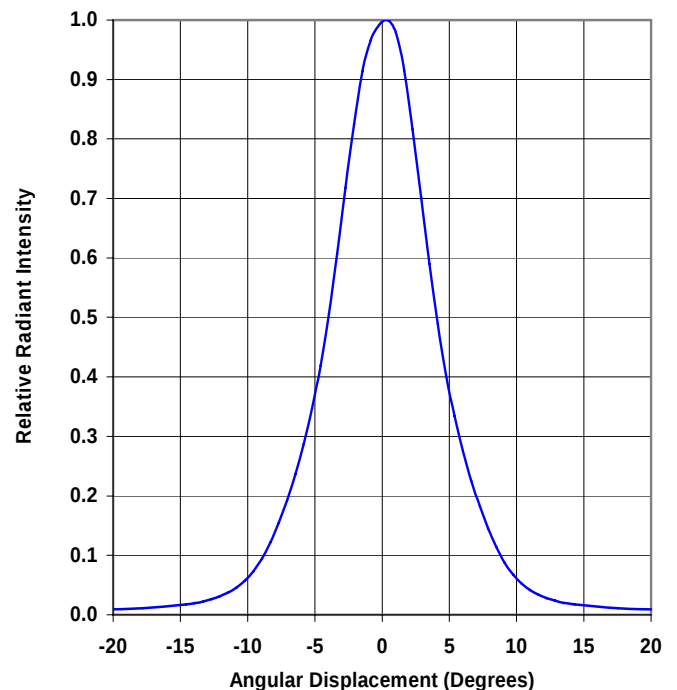
Beam Angle OP169 & OP269 Package
