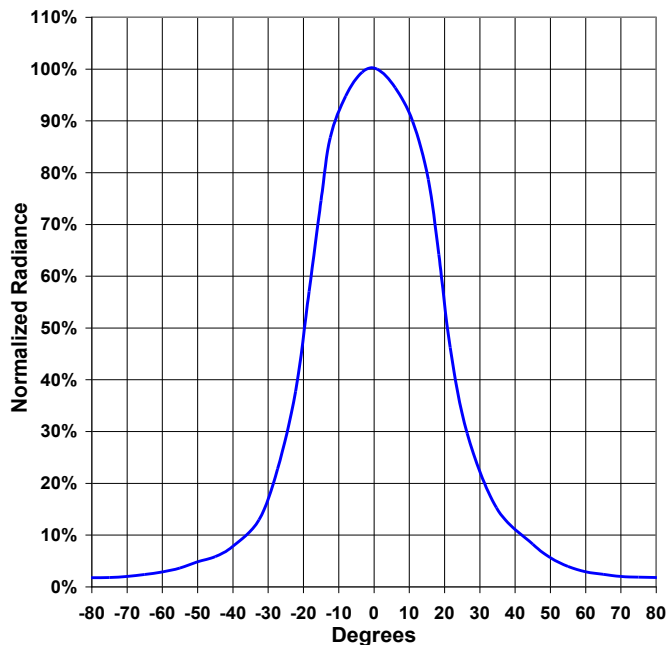
Beam Angle
