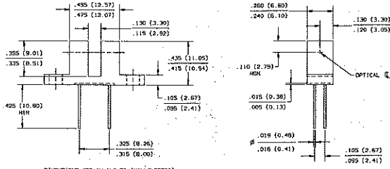
Package Configuration P
