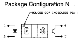
Package Configuration N
