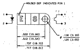
Package Configuration P
