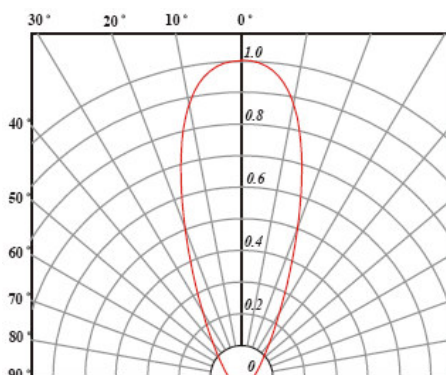
Radiation Pattern
