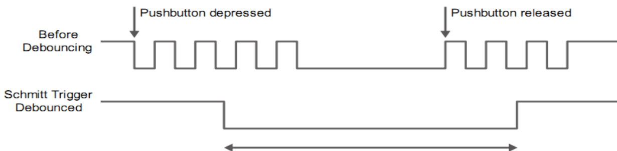
Figure 2-10 Push-button Debouncing
