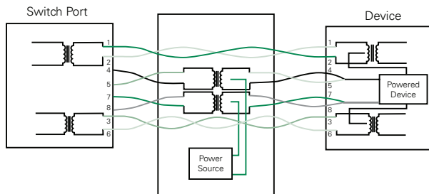
Figure 4.8 Mid-span Powering Technique
