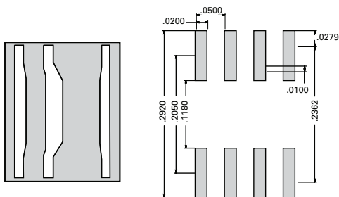
Figure 1.10 A: 5x6 QFN Footprint
