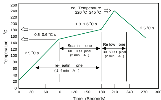
Figure 1.16: Reflow Soldering Profile for SN-Pb Soldering
