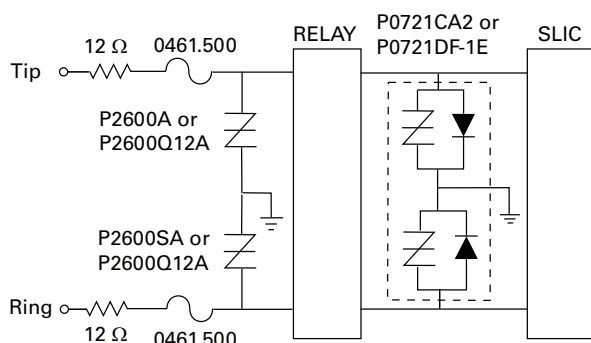
Figure 4.31 SLIC Protection with Fixed Voltage SIDACtor Devices
