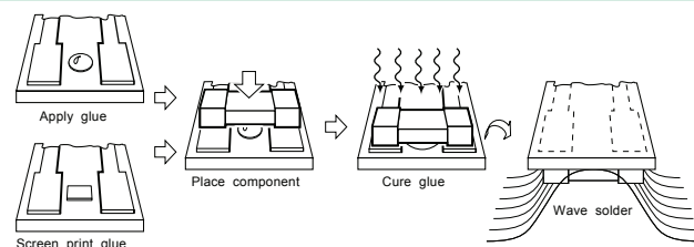
Figure 1.17: Wave Soldering of Surface Mount Components
