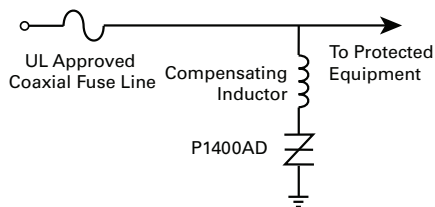
Figure 4.54 SIDACtor CATV Station Protection
