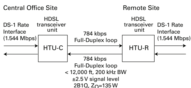
Figure 4.13 HDSL Overview
