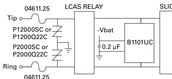
Figure 4.28 SLIC Protection with Battrax
