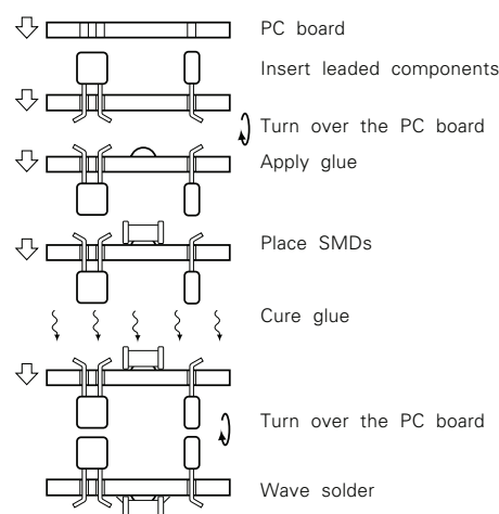
Figure 1.18: Wave Soldering of Surface Mount and Leaded Components
