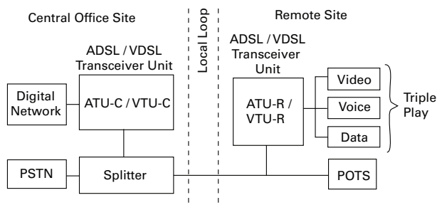
Figure 4.1 ADSL Overview
