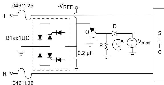
Figure 4.21 Battrax Protection Gate Buffer Circuit
