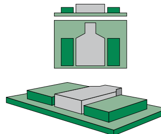
Figure 1.9: NSMD pad
