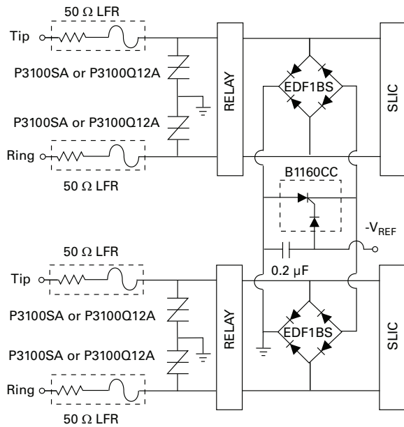
Figure 4.35 SLIC Protection with a Single Battrax Device
