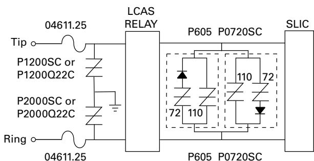
Figure 4.27 SLIC Protection with Asymmetrical Devices
