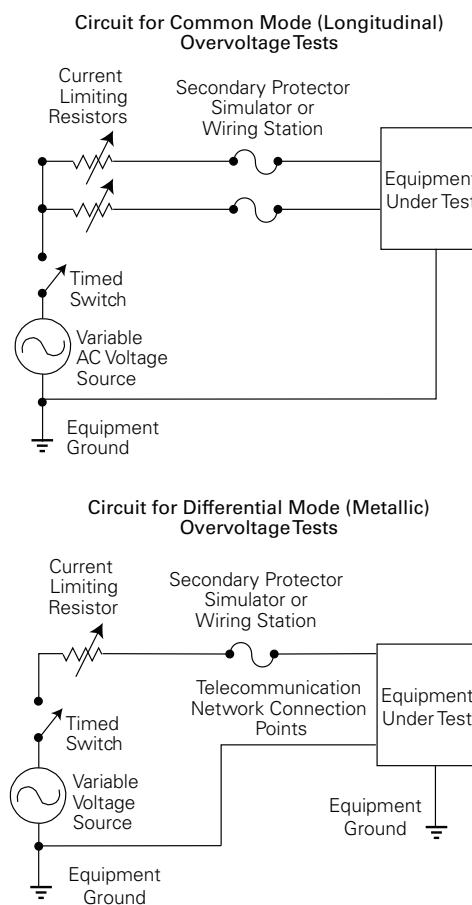
Figure 3.16 UL 497A Overvoltage Test
