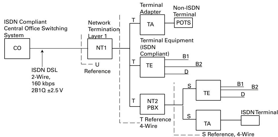
Figure 4.41 ISDN Protection
