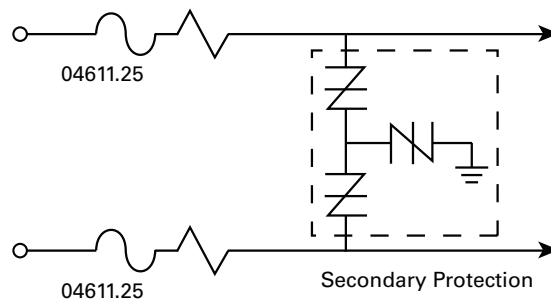
Figure 4.12 Coordination Solution with Resistor
