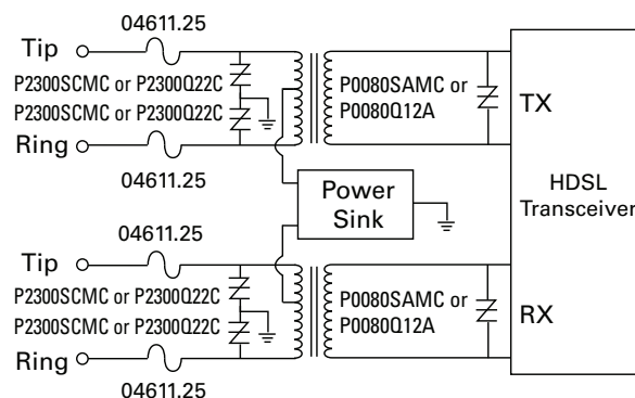
Figure 4.15 HDSL Quad Protection
