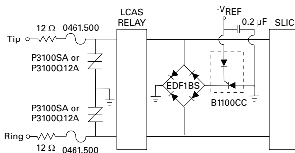
Figure 4.34 SLIC Protection with Single Battrax
