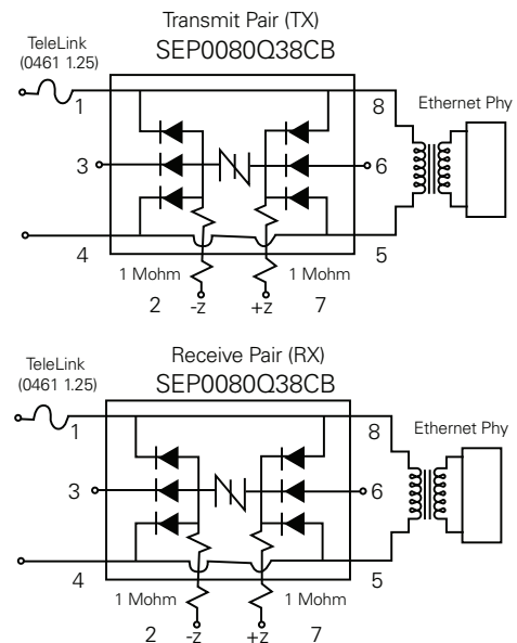
Figure 4.9 100BaseT Protection Circuit
