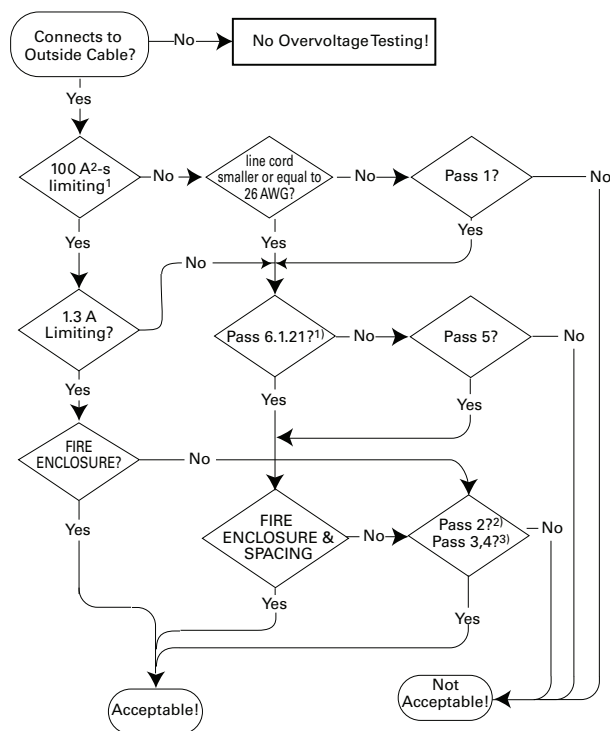
Figure 3.19 Overvoltage Flowchart
