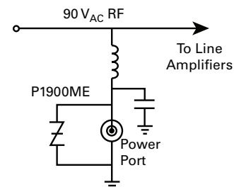
Figure 4.53 CATV Amplifier Protection
