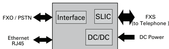
Figure 4.48 FXO connects to the PSTN.
