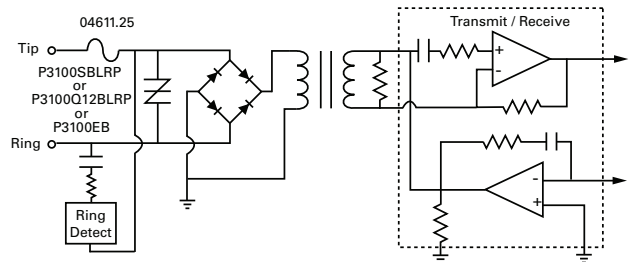
Figure 4.44 Modem Interface
