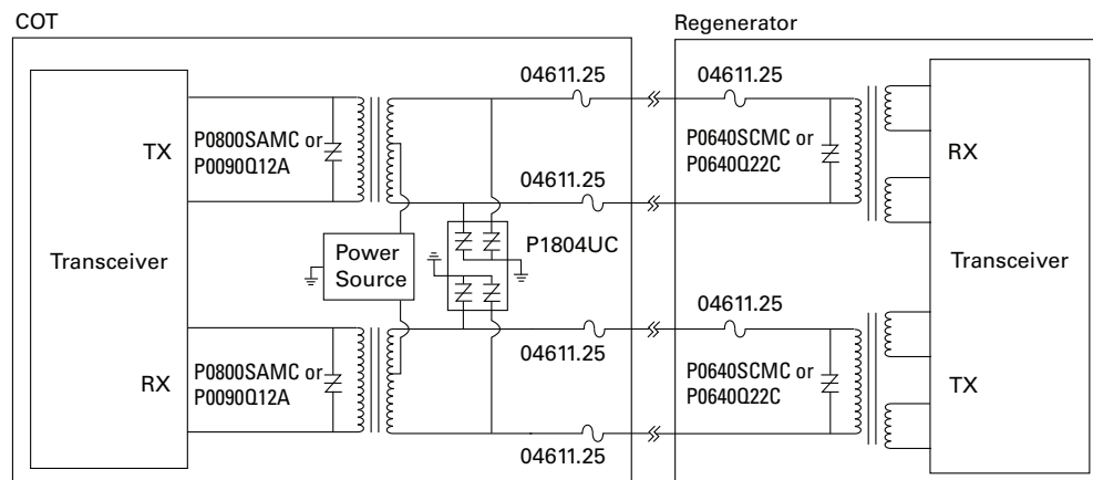
Figure 4.18 T1/E1/J1 Quad Protection
