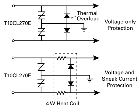
Figure 4.58 Balanced SIDACtor Primary Protection
