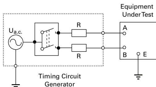
Figure 3.6 Connection Appearances (R = 10 \Omega , 20 \Omega , 40 \Omega , 80 \Omega , 160 \Omega , 300 \Omega , 600 \Omega , and 1000 \Omega for the various power fault tests)
