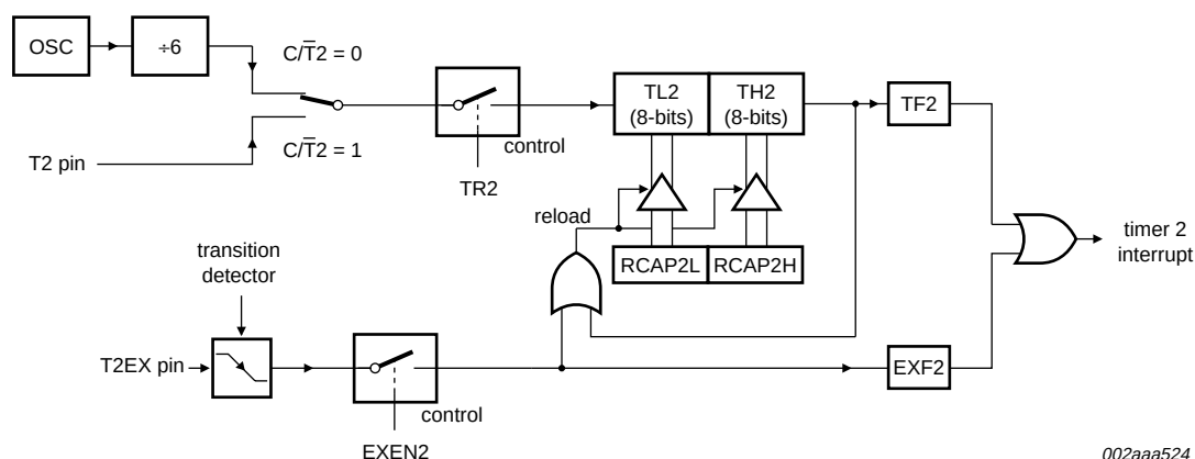
Fig 13. Timer 2 in auto-reload mode (DCEN = 0)
