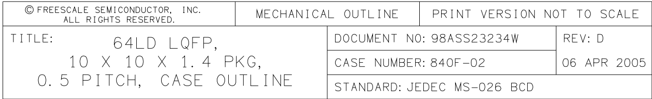
Figure 27. 64-pin LQFP Package Drawing (Case 840F, Doc #98ASS23234W), Sheet 1 of 3
