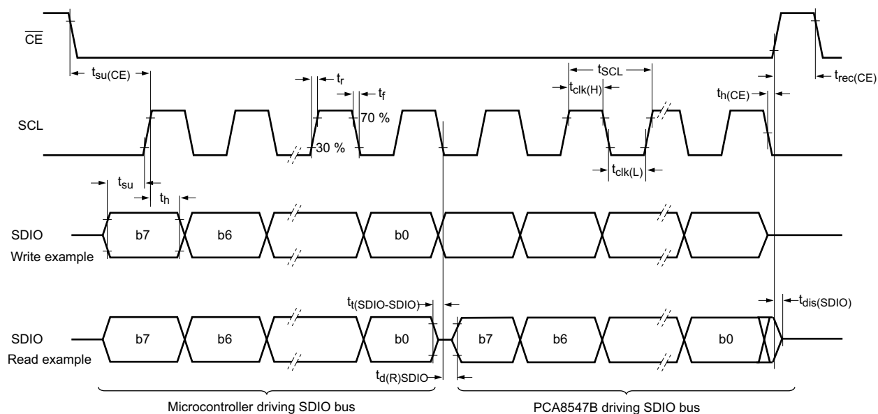
Fig 55. SPI-bus timing
