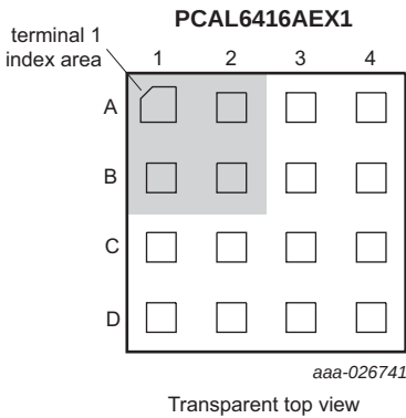
Fig 7. Pin configuration for X2QFN24 (2 mm × 2 mm); EX1 land grid array option
