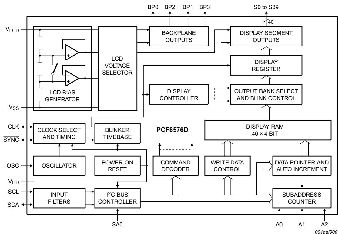
Fig 1. Block diagram of PCF8576D
