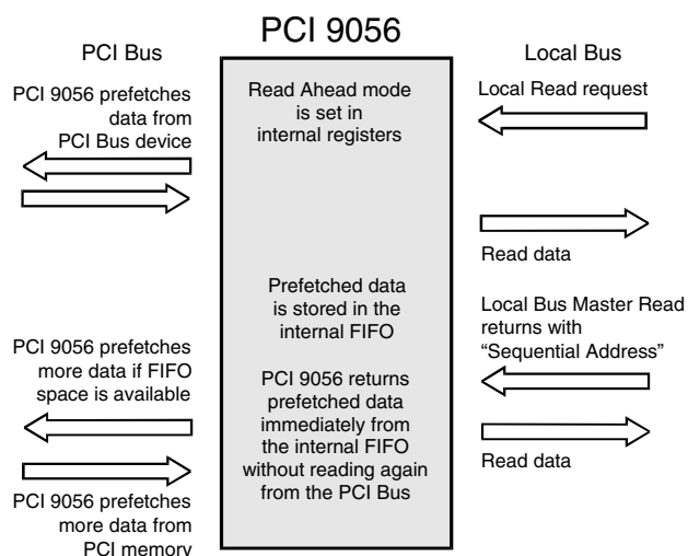
Figure 5-4. Direct Master Read Ahead Mode
