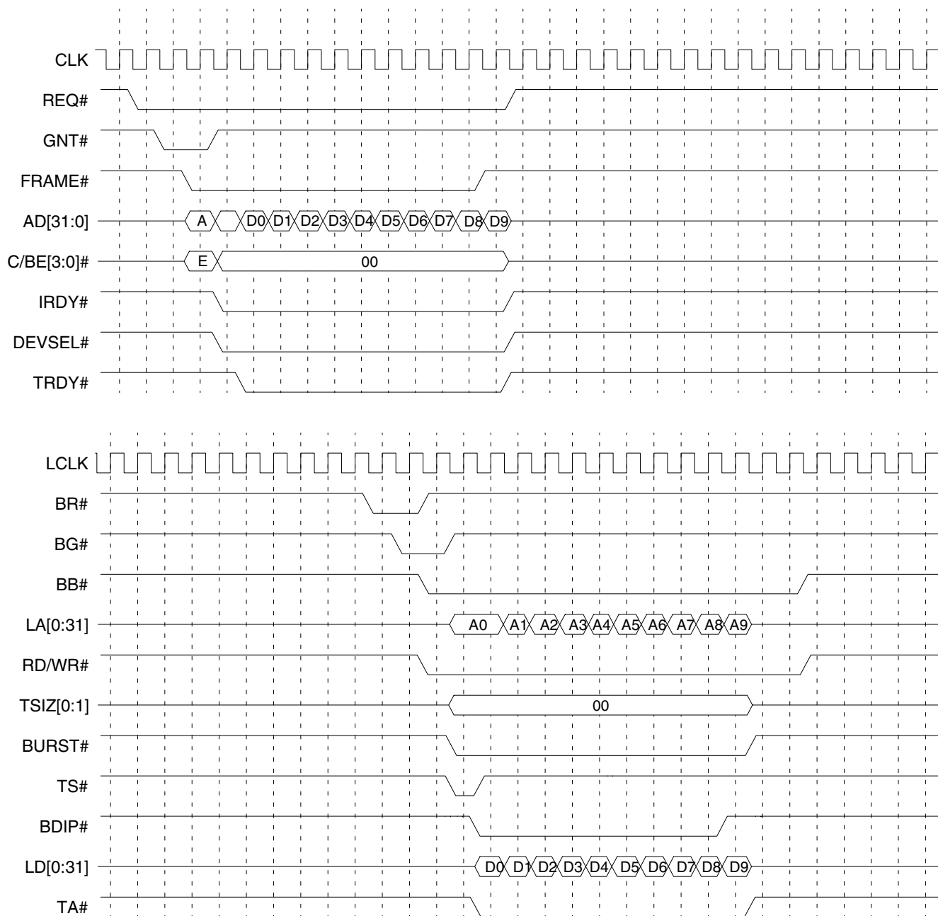
Timing Diagram 3-28. DMA PCI-to-Local, Continuous Burst Mode, Transfer Size = 10 Lwords
