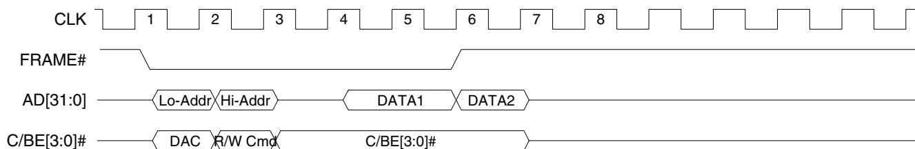
Figure 3-11. PCI Dual Address Cycle Timing
