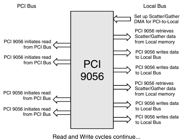
Figure 3-15. DMA Scatter/Gather Mode from PCI-to-Local Bus (Control Access from the Local Bus)
