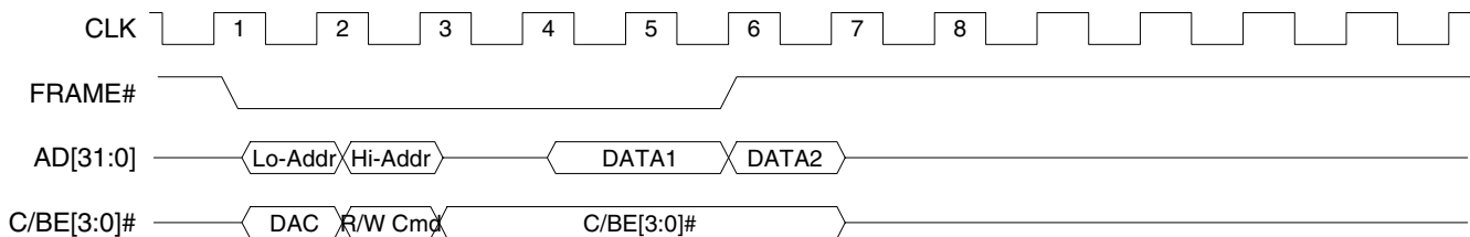
Figure 3-5. PCI Dual Address Cycle Timing
