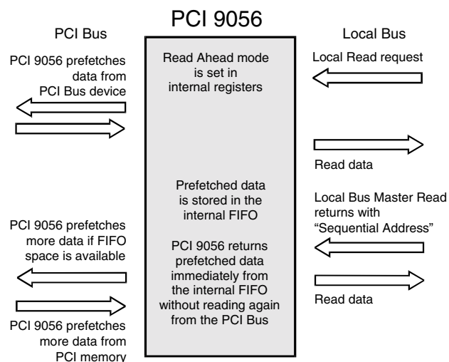
Figure 3-4. Direct Master Read Ahead Mode
