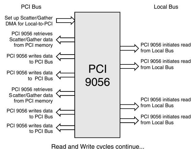
Figure 3-16. DMA Scatter/Gather Mode from Local-to-PCI Bus (Control Access from the PCI Bus)
