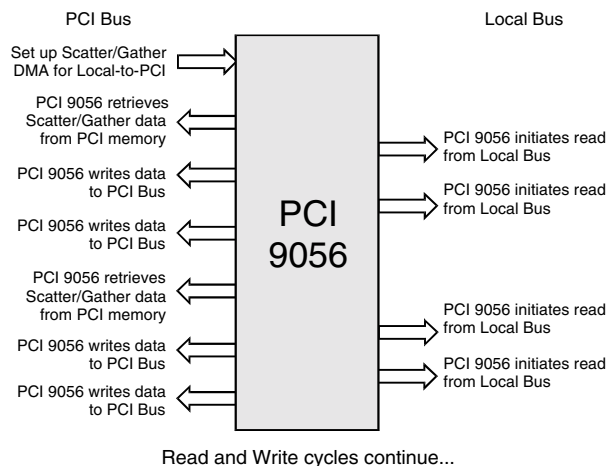
Figure 5-16. DMA Scatter/Gather Mode from Local-to-PCI Bus (Control Access from the PCI Bus)
