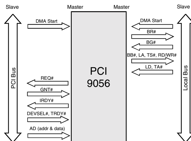
Figure 3-14. DMA, Local-to-PCI Bus
