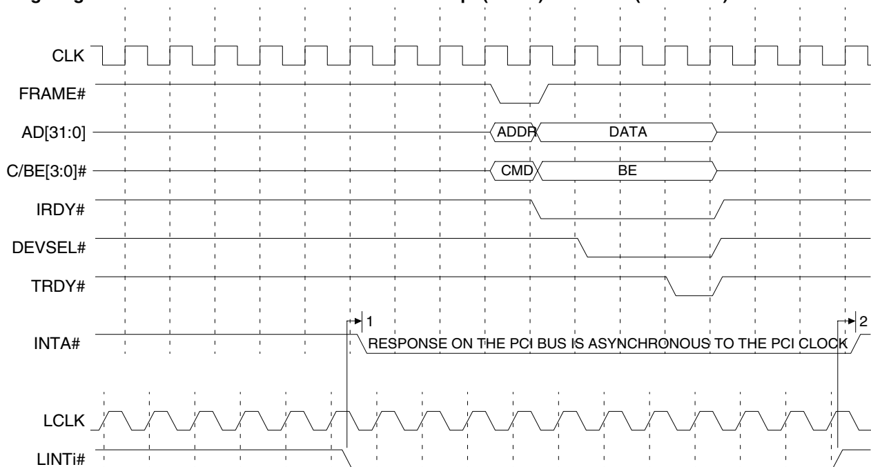
Timing Diagram 6-1. LINTi# Assertion Causes PCI Interrupt (INTA#) Assertion (All Modes)
