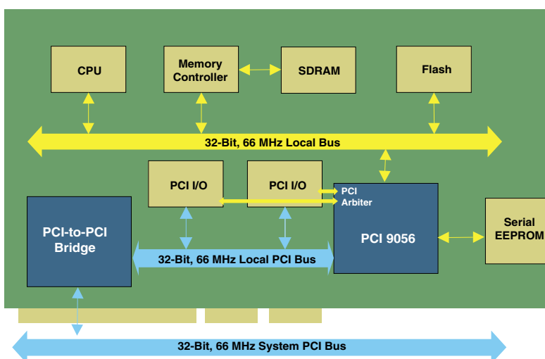
Figure 1-6. PCI 9056 PCI Adapter Card with Local PCI I/O and PCI-to-PCI Bridge
