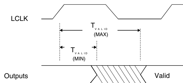
Figure 13-2. PCI 9056 Local Output Delay
