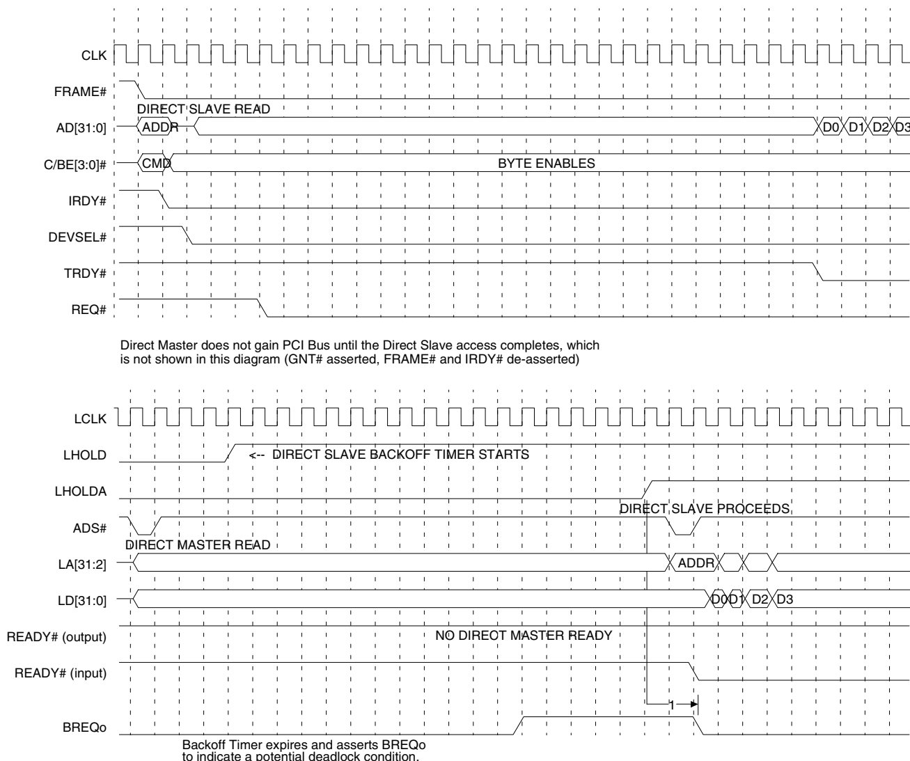
Timing Diagram 5-1. BREQo and Deadlock
