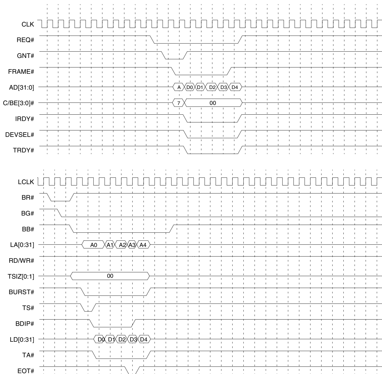
Timing Diagram 3-25. DMA Local-to-PCI, Continuous Burst Mode, with EOT# Assertion
