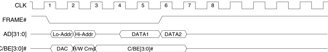
Figure 5-5. PCI Dual Address Cycle Timing
