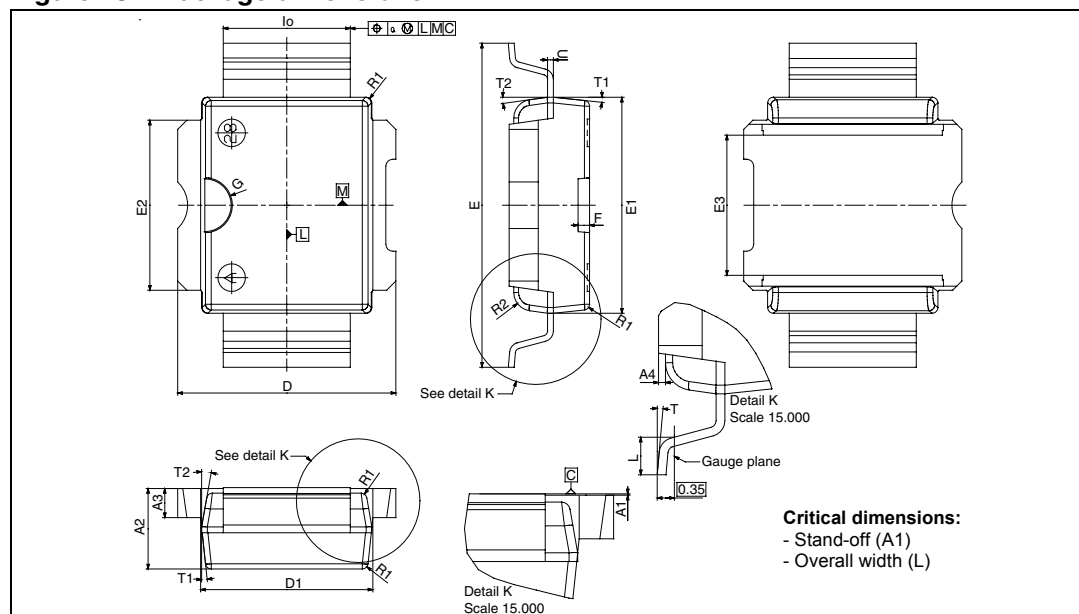
Figure 18. Package dimensions
