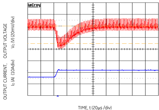
Figure 16. Transient Response to Dynamic Load Change from 50% to 100% at 12Vin, C_{out}=1x47\mu\text{F}+2x330\mu\text{F} , C_{Tune}=5600\text{pF} & R_{Tune}=270\text{ohms}
