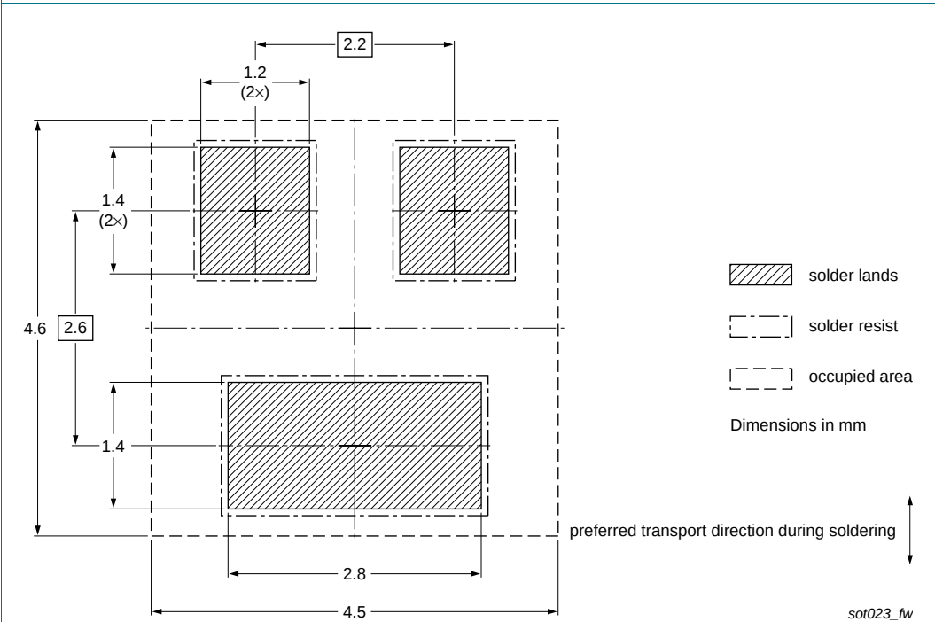
Fig 19. Wave soldering footprint PDTA114YT (SOT23)
