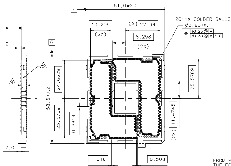
INTERSTITIAL BALL ARRANGEMENT
