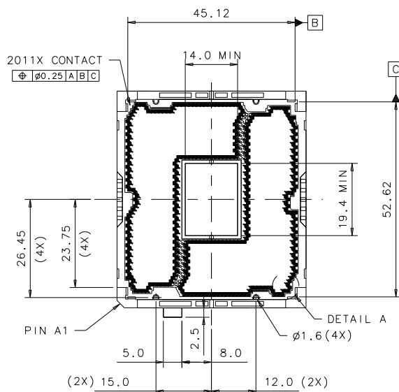
INTERSTITIAL PIN ARRANGEMENT
