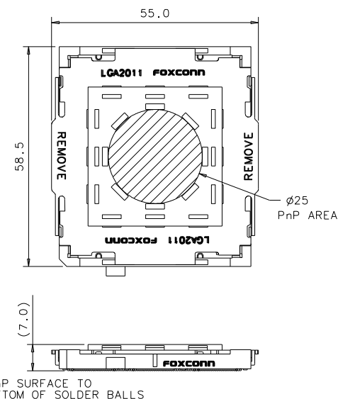
SOCKET W/ PICK-UP CAP
