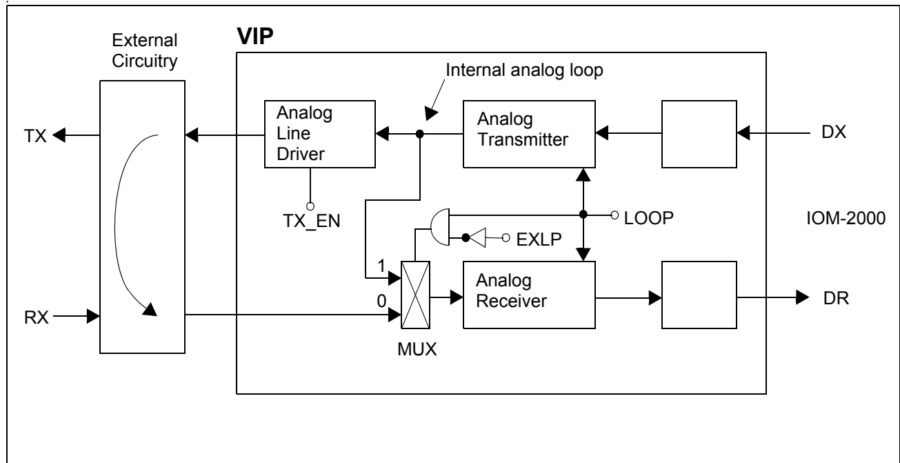
Figure 33 Internal and External Loop-Back Modes
