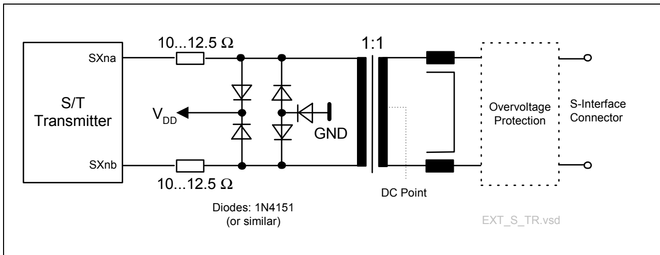
Figure 30 External S/T Transmitter Circuitry
