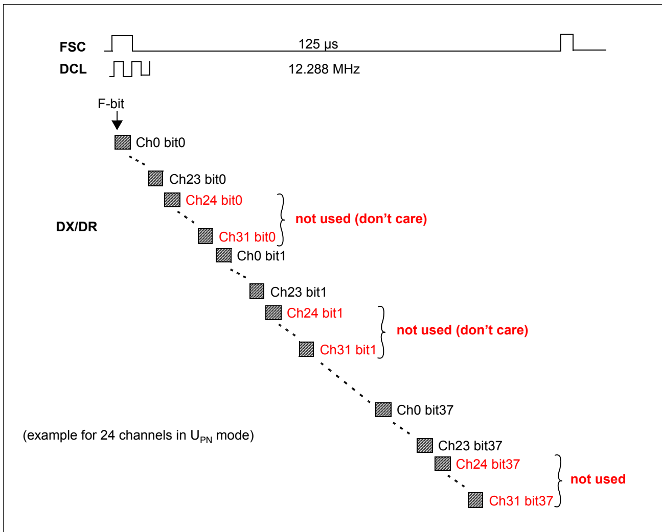
Figure 22 IOM-2000 Data Order (3 VIPs with 24 Channels)
