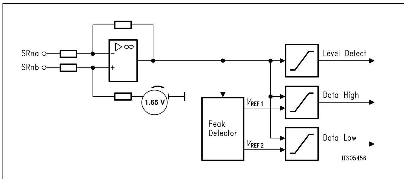
Figure 16 Receiver Functional Blocks
