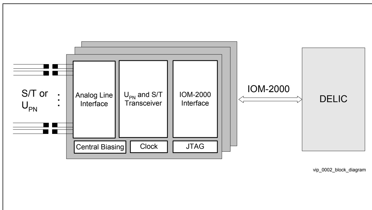
Figure 1 Top-Level Block Diagram of the VIP
