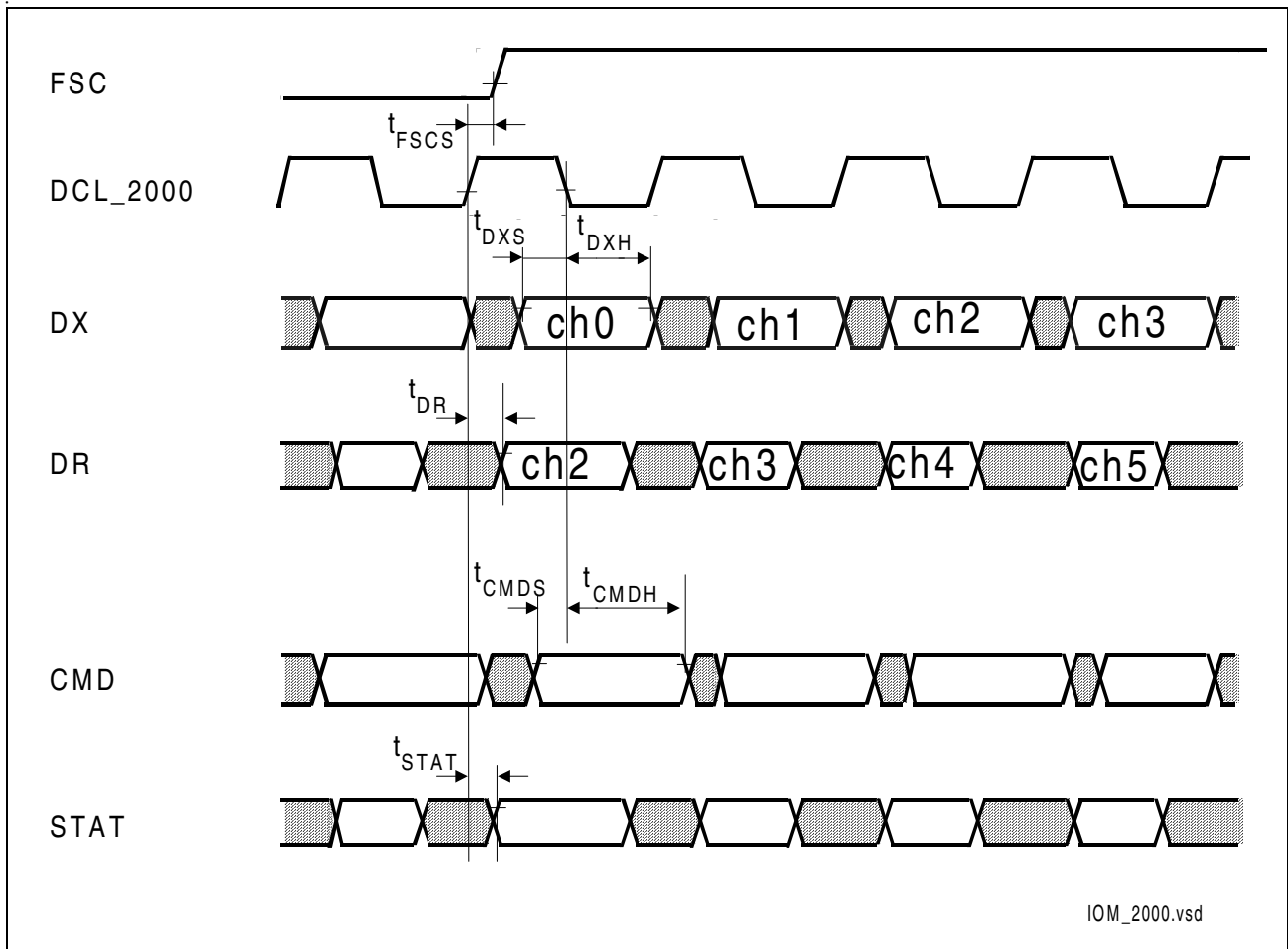
Figure 25 IOM-2000 Timing
