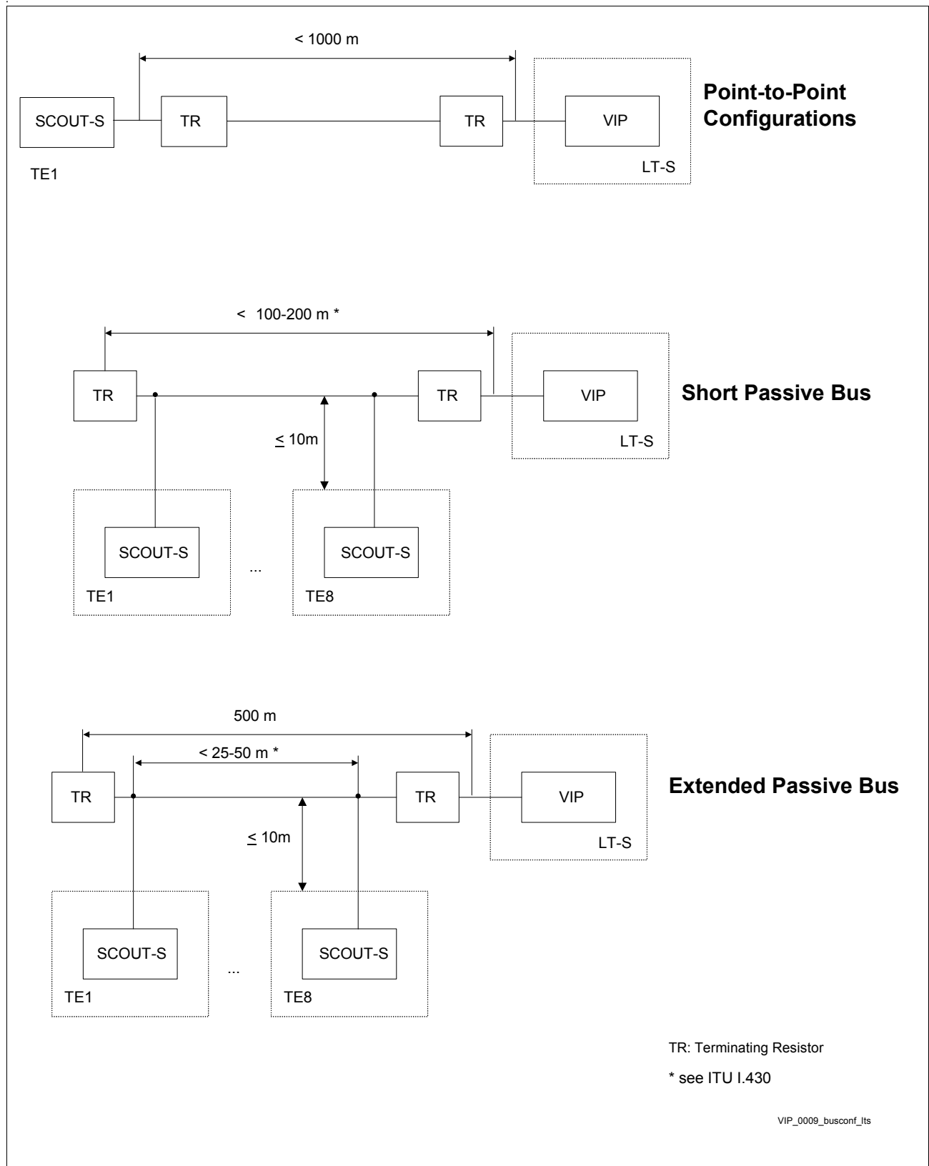
Figure 32 Wiring Configurations in User Premises (LT-S Mode)
