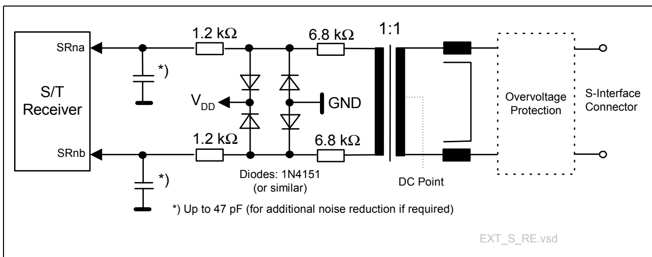
Figure 31 External S/T Receiver Circuitry
