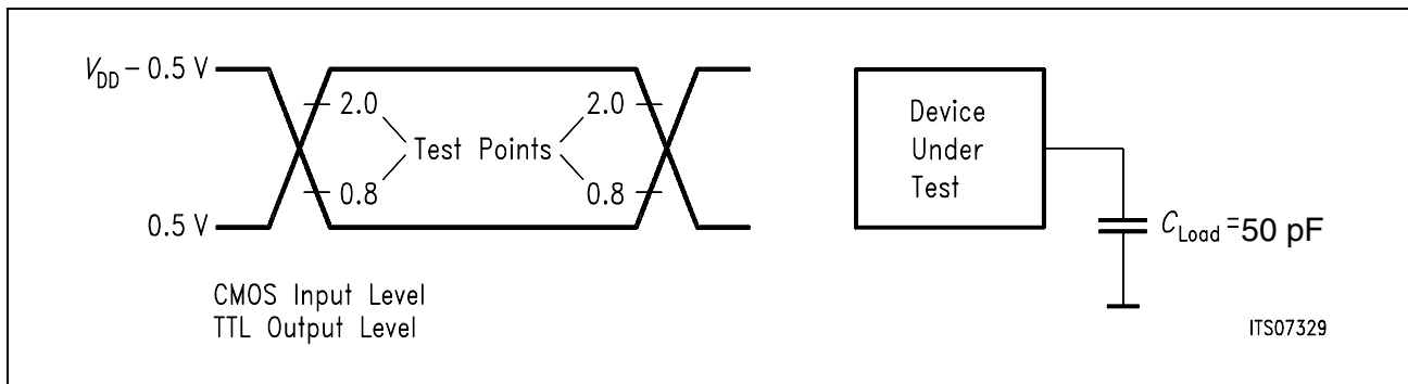
Figure 24 Input/Output Wave Form for AC Tests
