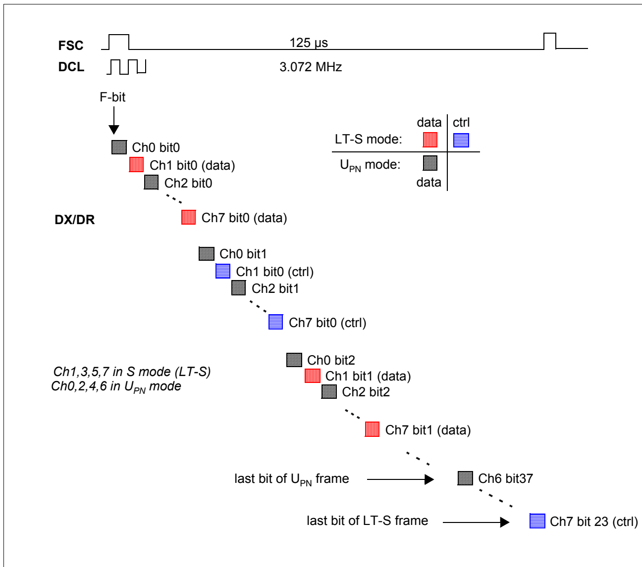
Figure 21 IOM-2000 Data Sequence (1 VIP with 8 Channels)
