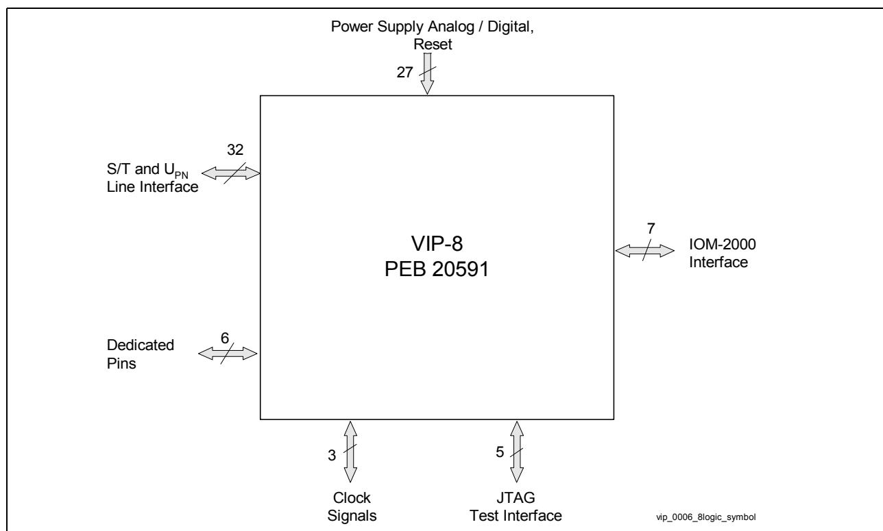
Figure 3 Logic Symbol PEB 20591
