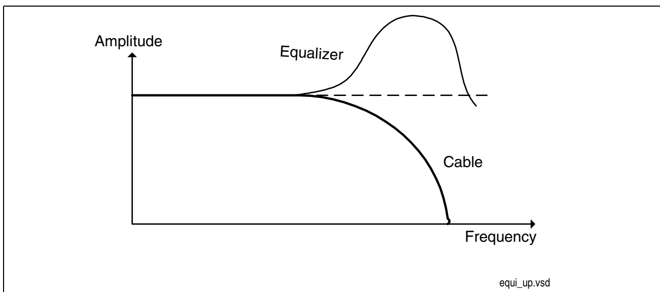
Figure 12 Equalizer Effect
