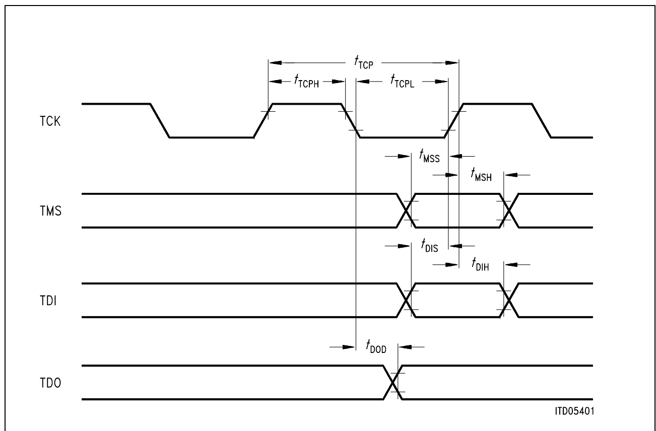
Figure 26 JTAG Timing
