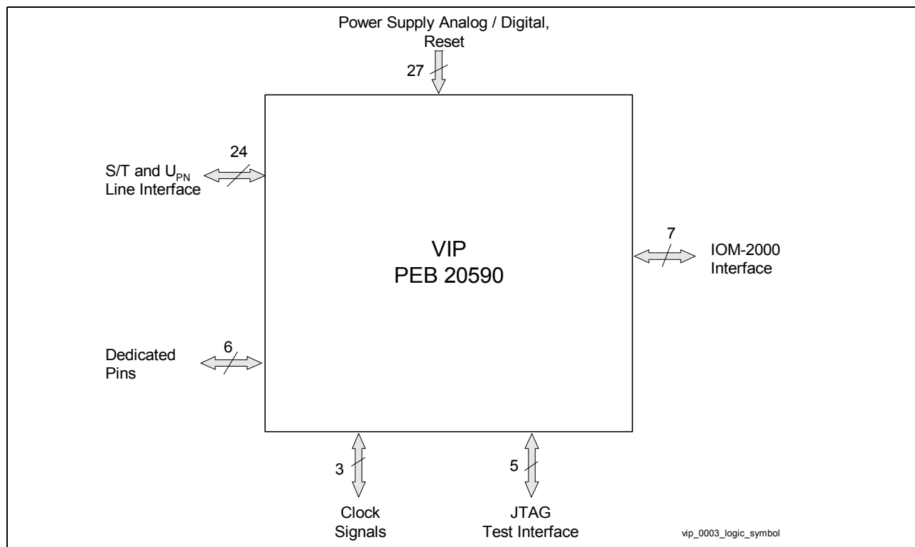
Figure 2 Logic Symbol PEB 20590 (72 of 80 Pins used)
