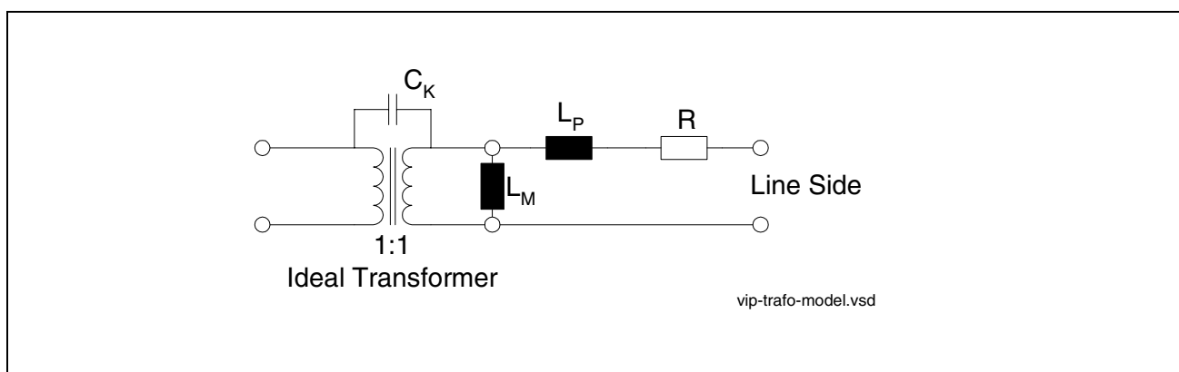
Figure 27 1:1 Transformer Model
