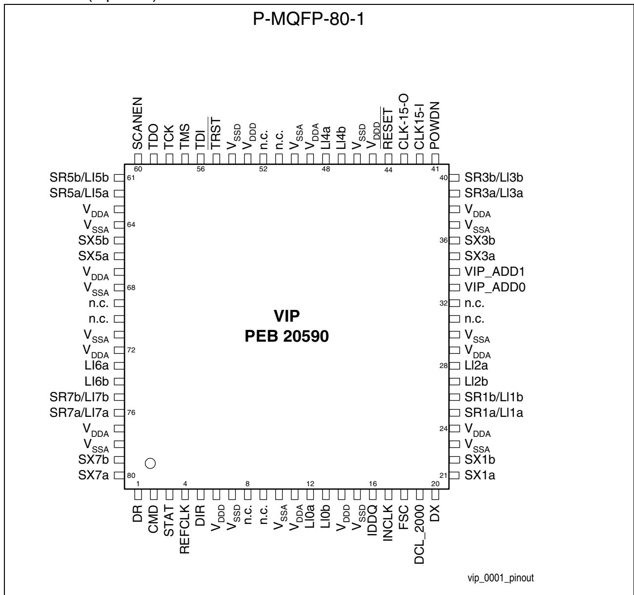
Figure 7 Pin Diagram, PEB 20590
