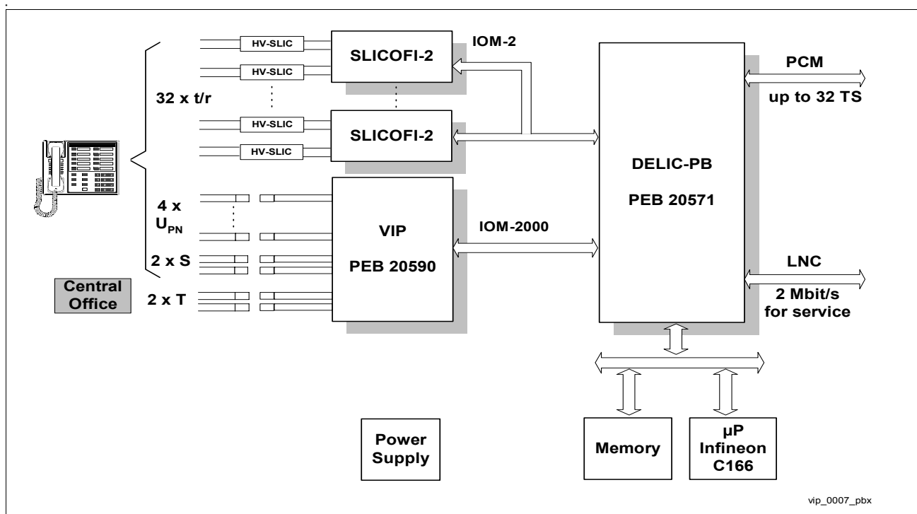
Figure 5 VIP in a Small PBX Solution
