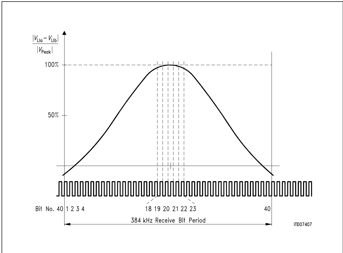
Figure 13 Receive Signal Oversampling on U_{PN} Interface
