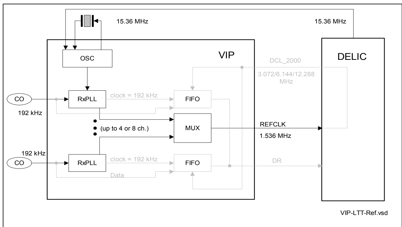
Figure 17 Clock Recovery in LT-T Mode
