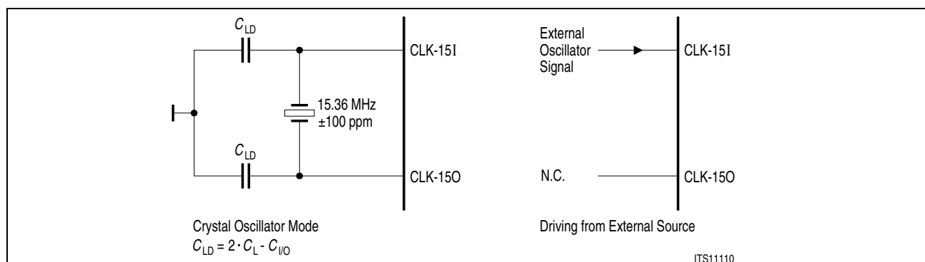
Figure 23 Recommended Oscillator Circuit
