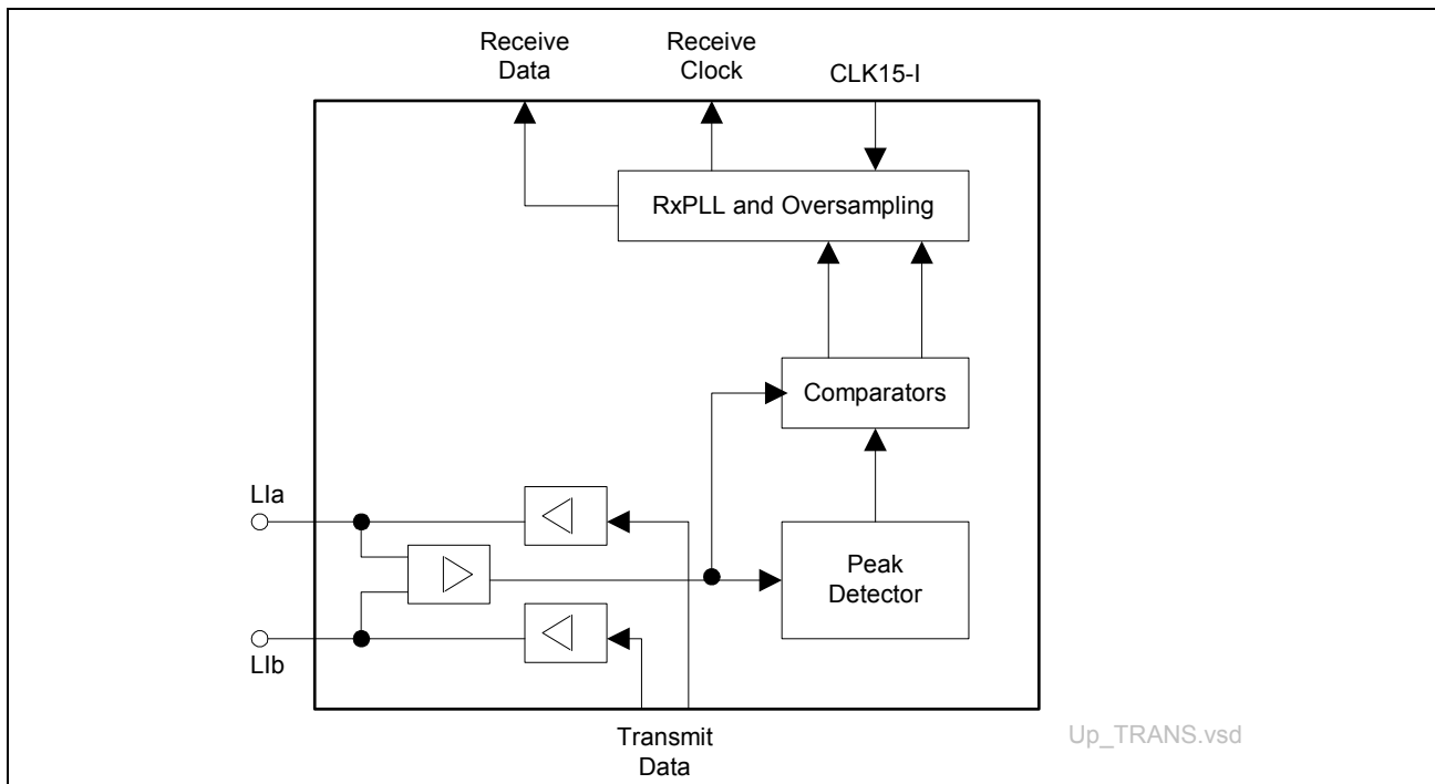
Figure 11 Transceiver Functional Blocks
