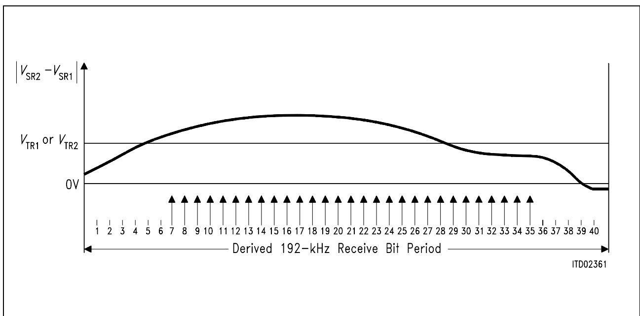
Figure 19 Receive Signal Oversampling in S/T Receiver
