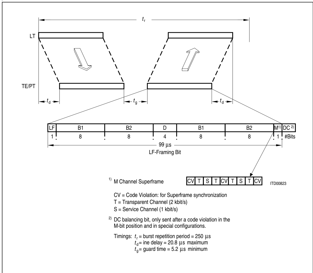
Figure 9 U_{PN} Interface Frame Structure
