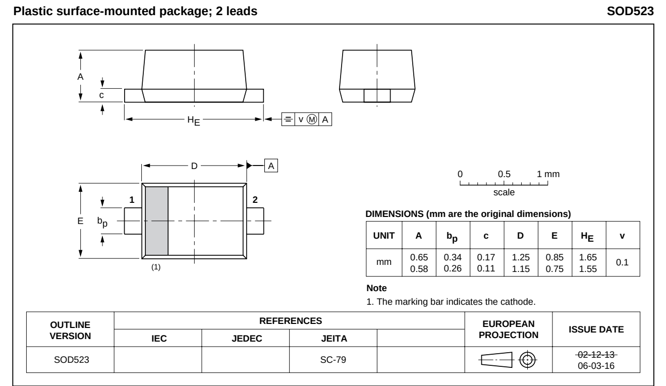
Fig 10. Package outline SOD523 (SC-79)
