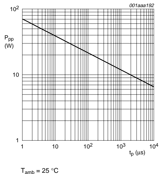
Fig 3. Peak pulse power as a function of exponential pulse duration t_p ; typical values
