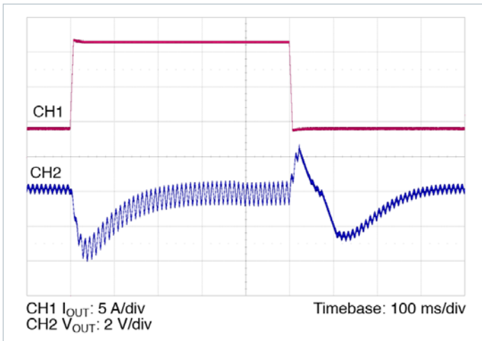
Figure 7 — Typical output voltage transient response, T_{CASE} = 30^{\circ}\text{C} , V_{IN} = 230\text{ V} , I_{OUT} = 16.7\text{ A} , 4.2\text{ A} C_{OUT} = 44,000\text{ }\mu\text{F}
