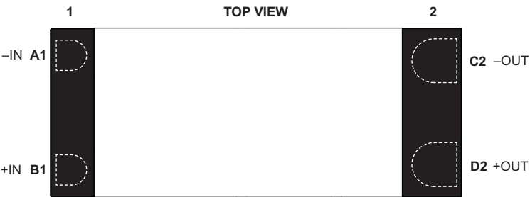
4414 VIA PFM - PCB Mount - Pins Down
