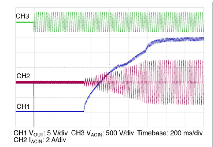
Figure 8 — Typical startup waveform, application of V_{IN} , R_{LOAD} = 1.4\text{ }\Omega , C_{OUT} = 44,000\text{ }\mu\text{F}
