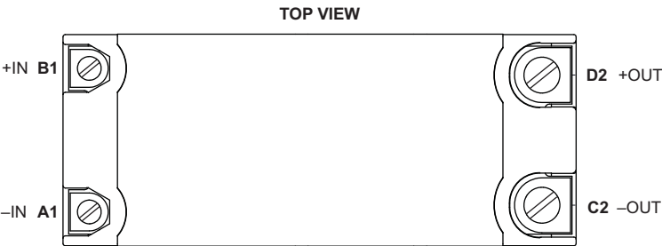
4414 VIA PFM - Chassis Mount - Terminals Up
