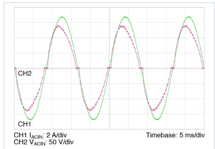
Figure 12 — Typical line current waveform, V_{IN} = 120\text{ V} , 60 HZ I_{OUT} = 16.7\text{ A} , C_{OUT} = 44,000\text{ }\mu\text{F}
