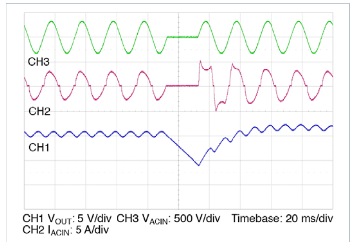
Figure 10 — Line drop out, 230 V 50 Hz, 0^{\circ} phase, I_{OUT} = 16.7\text{ A} , C_{OUT} = 44,000\text{ }\mu\text{F}
