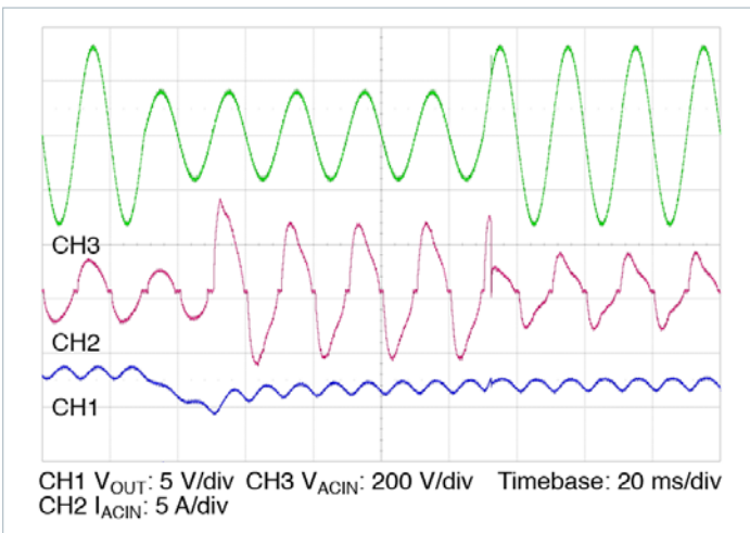
Figure 9 — 230 V, 120 V range change transient response, I_{OUT} = 16.7\text{ A} , C_{OUT} = 44,000\text{ }\mu\text{F}
