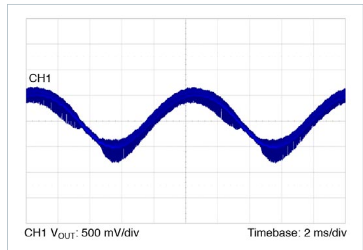
Figure 6 — Typical line frequency output voltage ripple waveform, T_{CASE} = 30^{\circ}\text{C} , V_{IN} = 230\text{ V} , I_{OUT} = 16.7\text{ A} , C_{OUT} = 44,000\text{ }\mu\text{F} , 20 MHz BW
