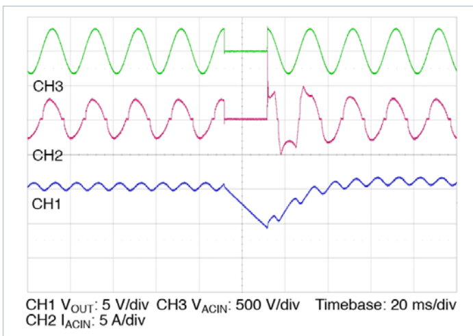
Figure 11 — Line drop out, 90^{\circ} phase, V_{IN} = 230\text{ V} , I_{OUT} = 16.7\text{ A} , C_{OUT} = 44,000\text{ }\mu\text{F}
