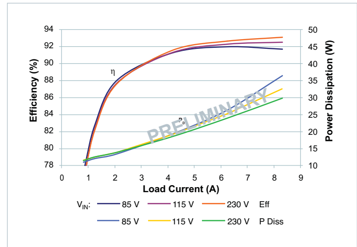
Figure 18 — V_{IN} to V_{OUT} efficiency and power dissipation vs. V_{IN} and I_{OUT} , T_{CASE} = 20^{\circ}\text{C}
