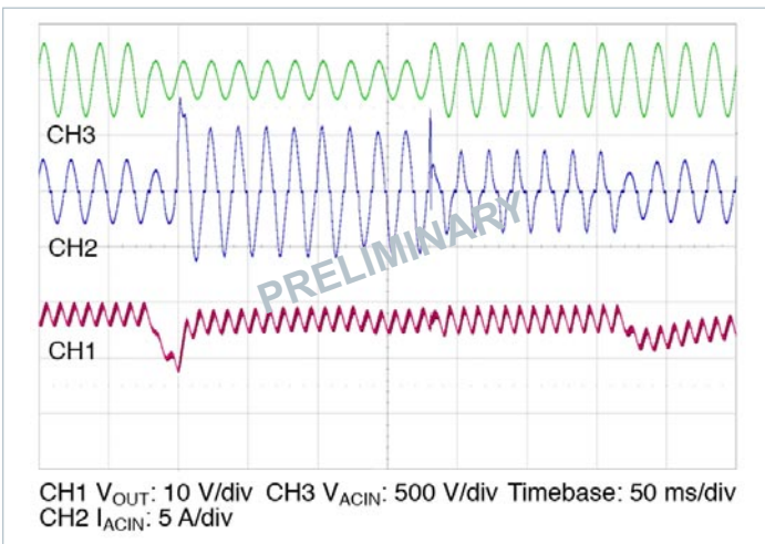
Figure 9 — 230 V, 120 V range change transient response, I_{OUT} = 8.3\text{ A} , C_{OUT} = 10,000\text{ }\mu\text{F}
