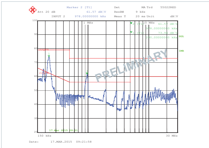
Figure 15 — Typical EMI Spectrum, Peak Scan, 90% load, 230 V_{IN} , C_{OUT} = 10,000 \mu F, No Inlet Filter
