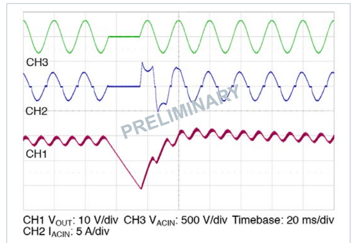
Figure 10 — Line drop out, 230 V 50 Hz, 0^{\circ} phase, I_{OUT} = 8.3\text{ A} , C_{OUT} = 10,000\text{ }\mu\text{F}
