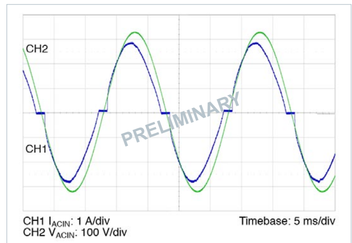
Figure 12 — Typical line current waveform, V_{IN} = 120\text{ V} , 60\text{ HZ} I_{OUT} = 8.3\text{ A} , C_{OUT} = 10,000\text{ }\mu\text{F}
