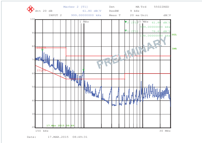
Figure 13 — Typical EMI Spectrum, Peak Scan, 90% load, 115 V_{IN} , C_{OUT} = 10,000 \mu F, No Inlet Filter
