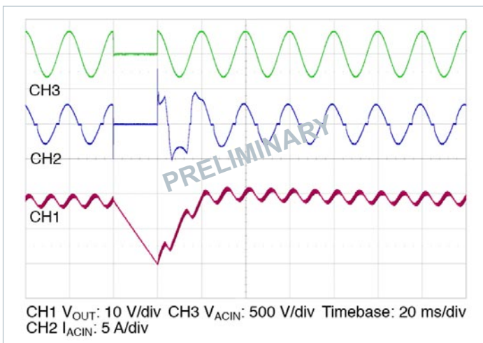
Figure 11 — Line drop out, 90^{\circ} phase, V_{IN} = 230\text{ V} , I_{OUT} = 8.3\text{ A} , C_{OUT} = 10,000\text{ }\mu\text{F}
