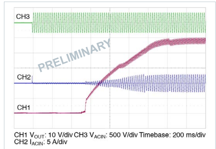
Figure 8 — Typical startup waveform, application of V_{IN} , R_{LOAD} = 5.7\text{ }\Omega , C_{OUT} = 10,000\text{ }\mu\text{F}
