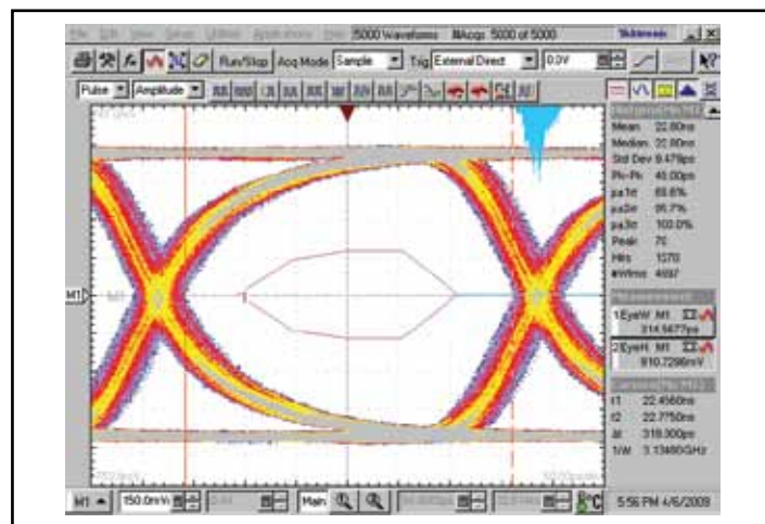
Output Eye Diagram (2.7Gbps, 1200mV)
