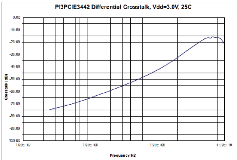
Differential Crosstalk
