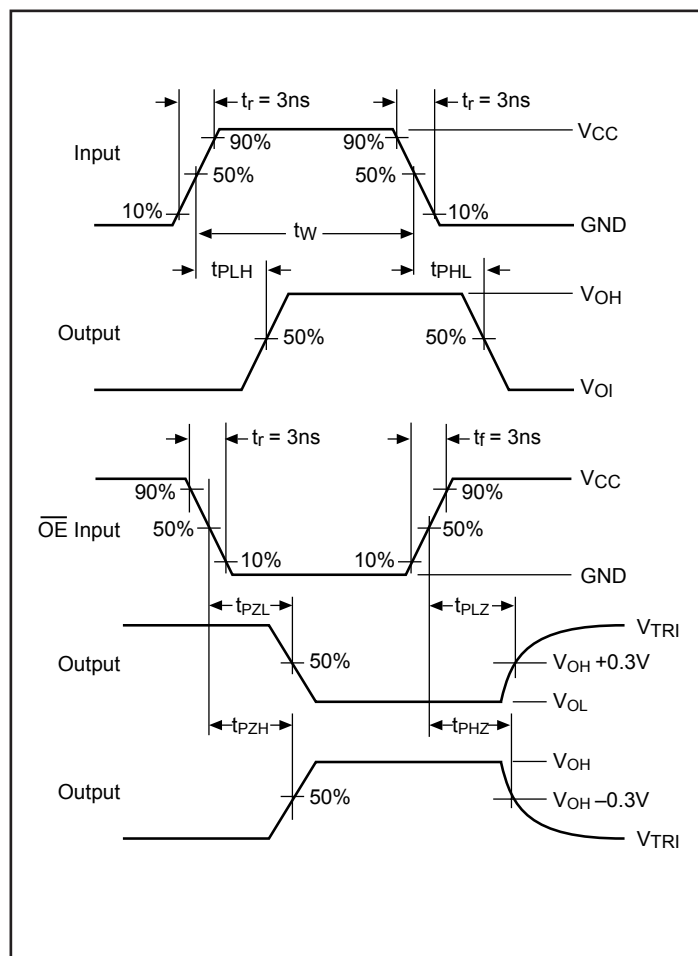
Figure 3. AC Waveforms
