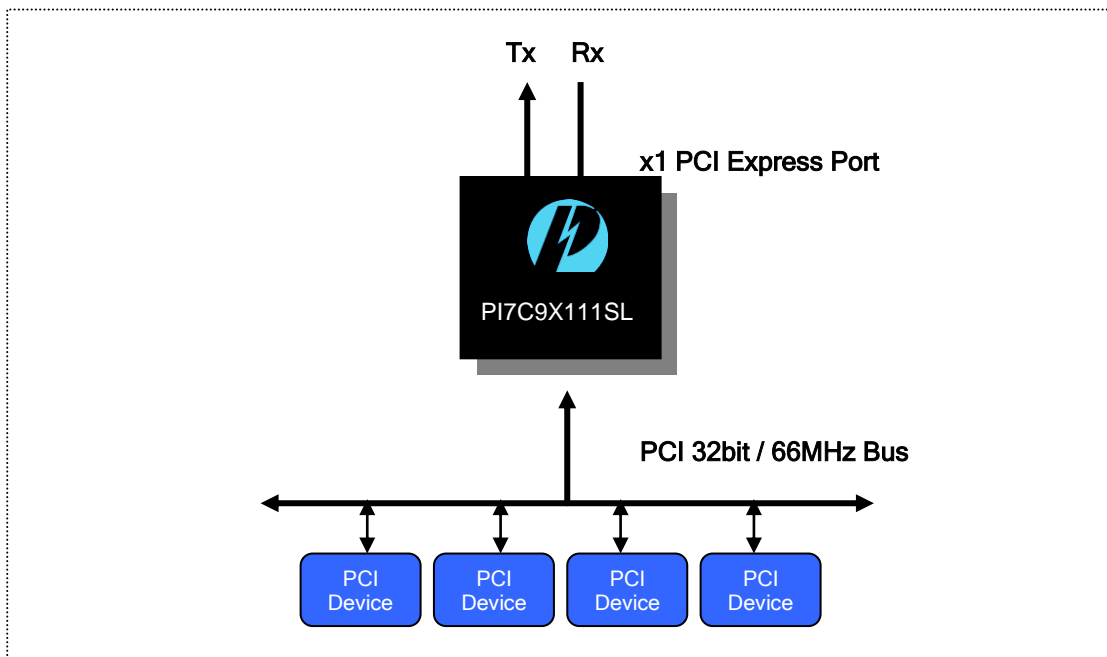
Figure 1-1 PI7C9X111SL Topology
