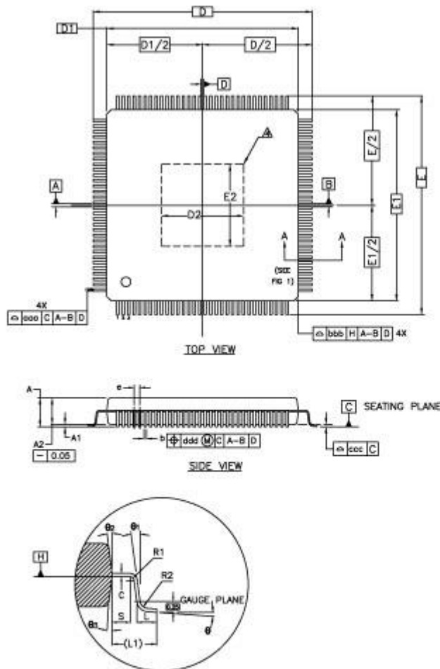
Figure 16-1 Package Outline Drawing
