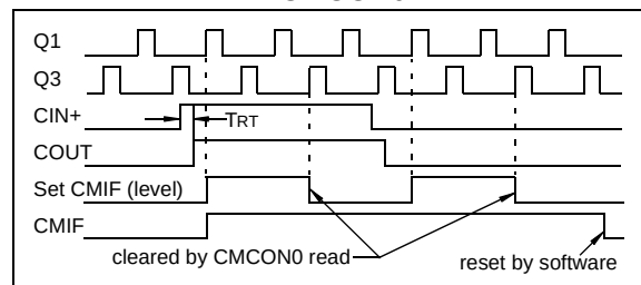
FIGURE 8-6: COMPARATOR INTERRUPT TIMING WITH CMCON0 READ
