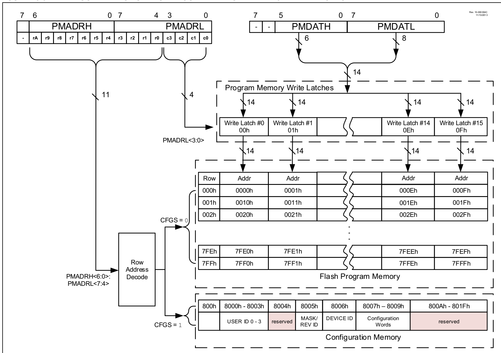
PIC12(L)F1612/16(L)F1613
