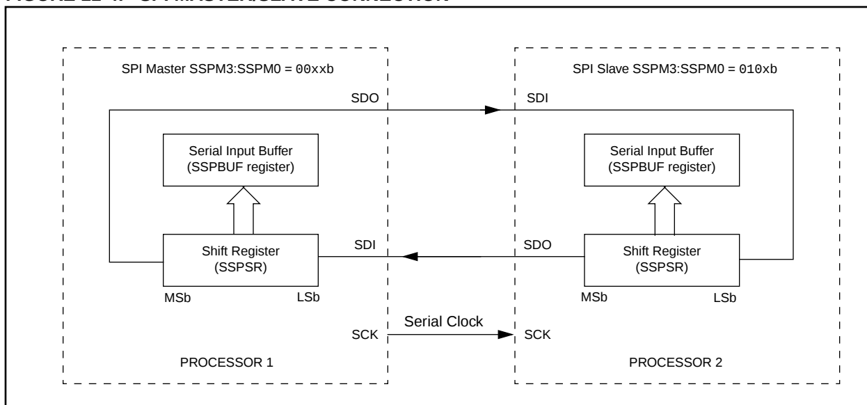
FIGURE 11-4: SPI MASTER/S�AVE CONNECTION
