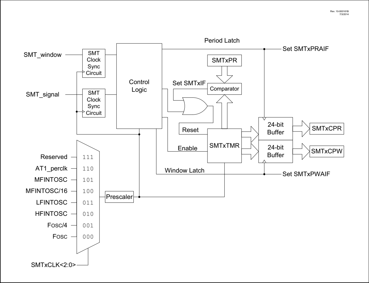
FIGURE 30-2: SMT SIGNAL AND WINDOW BLOCK DIAGRAM
