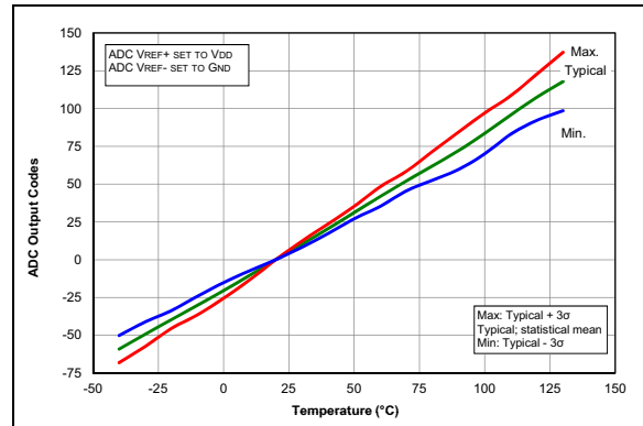
FIGURE 36-76: Temp. Indicator Slope Normalized to 20^\circ\text{C} , High Range, V_{DD} = 5.5V , PIC16F1614/8 Only.
