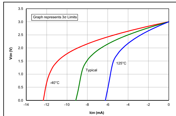
FIGURE 36-41: V_{OH} vs. I_{OH} Over Temperature, V_{DD} = 3.0V .
