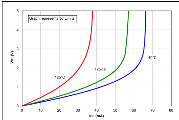
FIGURE 36-38: V_{OL} vs. I_{OL} Over Temperature, V_{DD} = 5.0V , PIC16F1614/8 Only.
