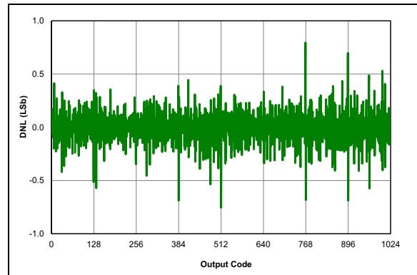
FIGURE 36-65: ADC 10-bit Mode, Single-Ended DNL, V_{DD} = 3.0V , T_{AD} = 1\text{ }\mu\text{s} , 25^\circ\text{C} .
