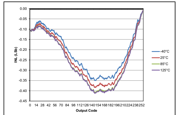
FIGURE 36-95: Typical DAC INL Error, V_{DD} = 5.0V , V_{REF} = \text{External } 5V , PIC16F1614/8 Only.
