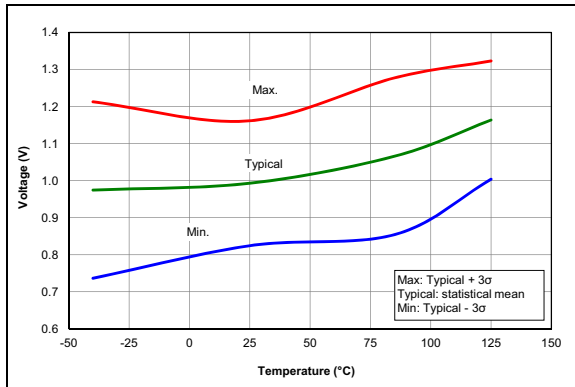
FIGURE 36-61: POR Rearm Voltage, NP Mode, PIC16LF1614/8 Only.
