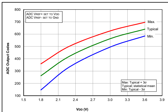
FIGURE 36-75: Temp. Indicator Initial Offset, Low Range, Temp. = 20^\circ\text{C} , PIC16LF1614/8 Only.
