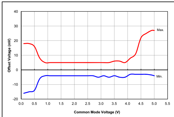
FIGURE 36-87: Comparator Offset, NP Mode ( CxSP = 1 ), V_{DD} = 5.5V , Typical Measured Values From -40^\circ C to 125^\circ C , PIC16F1614/8 Only.
