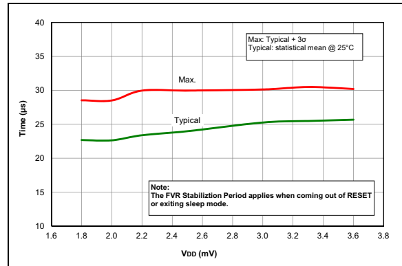
FIGURE 36-64: FVR Stabilization Period, PIC16LF1614/8 Only.
