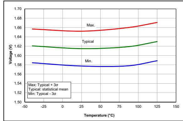
FIGURE 36-59: POR Release Voltage.
