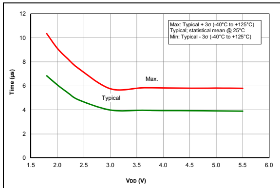
FIGURE 36-62: Wake From Sleep, VREGPM = 0.
