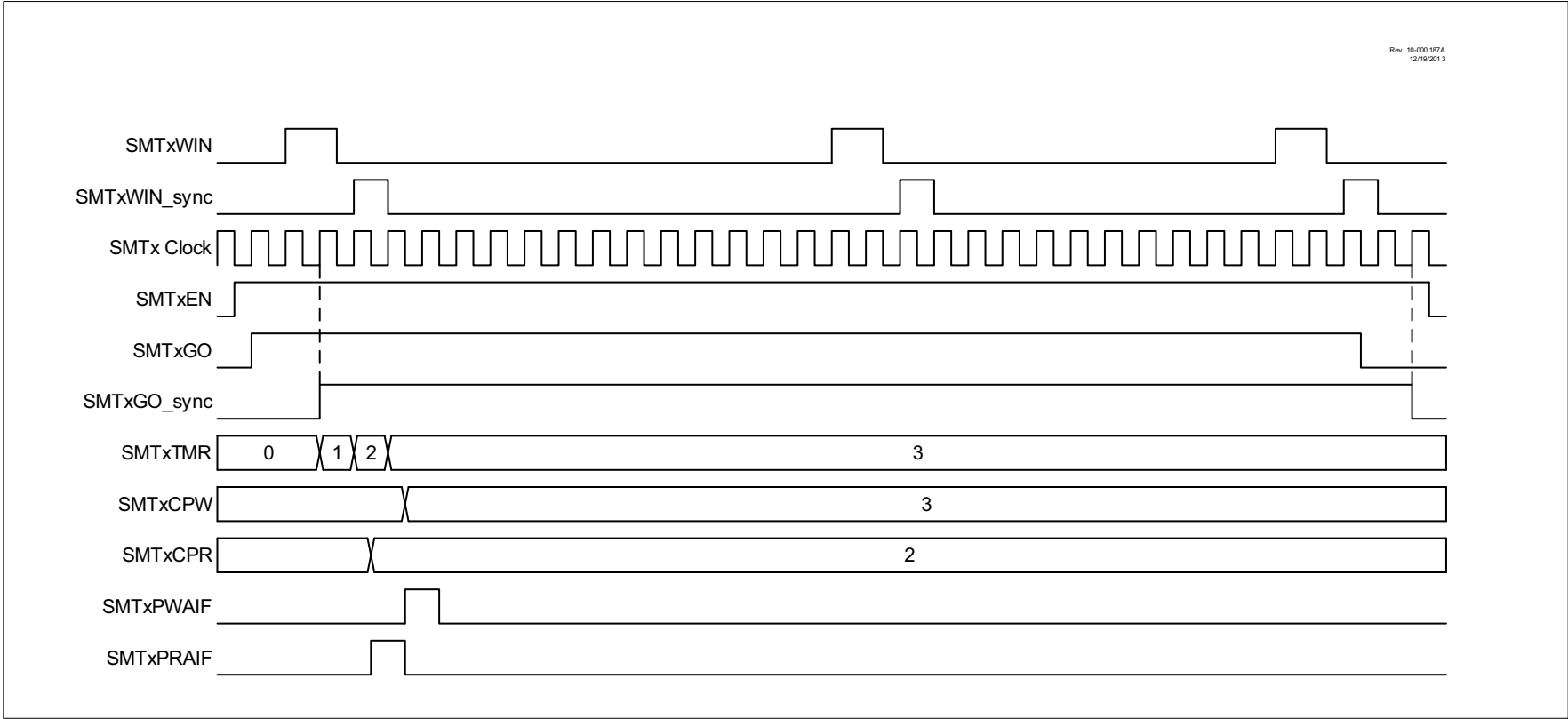
FIGURE 30-17: CAPTURE MODE SINGLE ACQUISITION TIMING DIAGRAM
