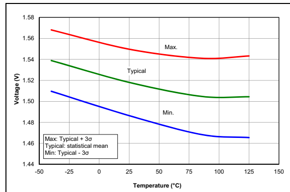
FIGURE 36-60: POR Rearm Voltage, NP Mode ( V_{REGPM1} = 0 ), PIC16F1614/8 Only.
