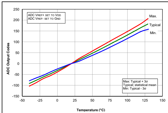
FIGURE 36-81: Temp. Indicator Slope Normalized to 20^\circ\text{C} , High Range, V_{DD} = 3.6V , PIC16LF1614/8 Only.
