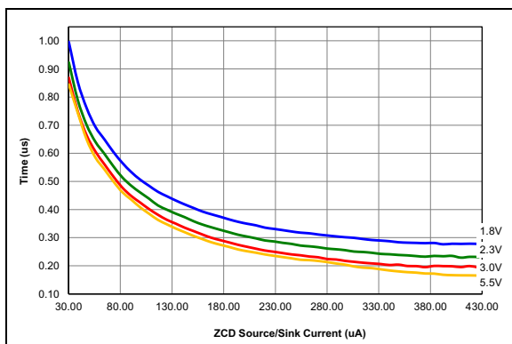
FIGURE 36-104: ZCD Pin Response Timer over Current, Typical Measured Values from -40^\circ\text{C} to 125^\circ\text{C} .
