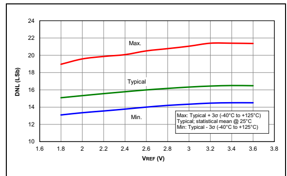
FIGURE 36-96: DAC INL Error, V_{DD} = 3.0V .
