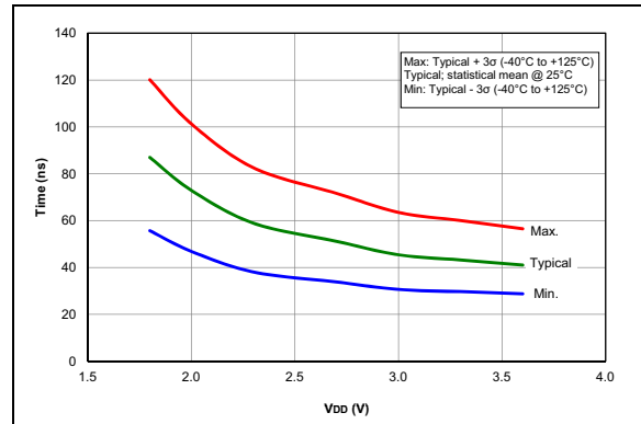
FIGURE 36-88: Comparator Response Time Over Voltage, NP Mode ( CxSP = 1 ), Typical Measured Values, PIC16LF1614/8 Only.
