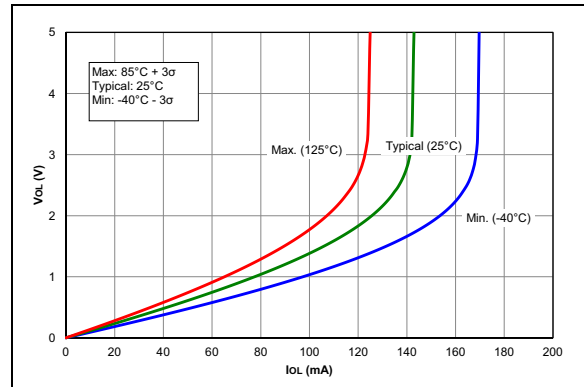
FIGURE 36-40: V_{OL} vs. I_{OL} Over Temperature for High Drive Pins, V_{DD} = 5.0V , PIC16F1614/8 Only.
