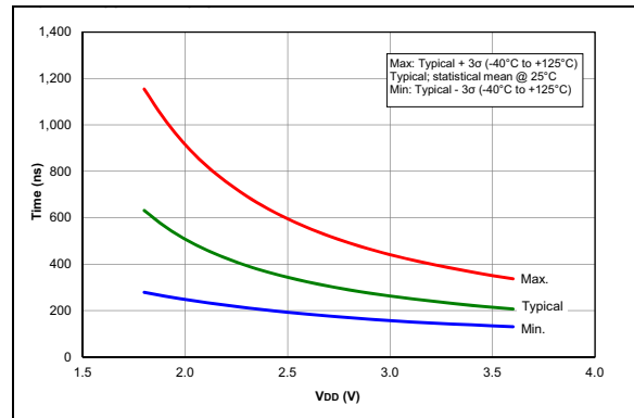
FIGURE 36-90: Comparator Output Filter Delay Time Over Temp., NP Mode ( CxSP = 1 ), Typical Measured Values, PIC16LF1614/8 Only.
