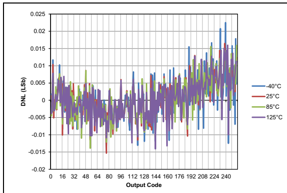
FIGURE 36-92: Typical DAC DNL Error, V_{DD} = 3.0V , V_{REF} = \text{External } 3V .
