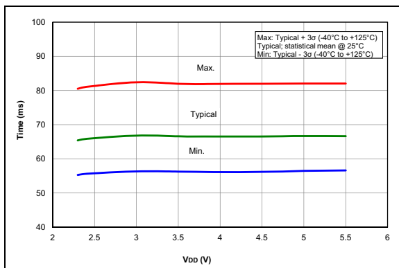
FIGURE 36-57: PWRT Period, PIC16F1614/8 Only.
