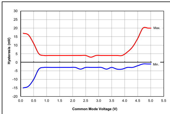
FIGURE 36-86: Comparator Offset, NP Mode ( CxSP = 1 ), V_{DD} = 5.0V , Typical Measured Values at 25^\circ C , PIC16F1614/8 Only.
