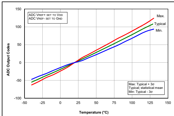
FIGURE 36-80: Temp. Indicator Slope Normalized to 20^\circ\text{C} , Low Range, V_{DD} = 3.0V , PIC16LF1614/8 Only.
