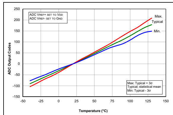
FIGURE 36-77: Temp. Indicator Slope Normalized to 20^\circ\text{C} , High Range, V_{DD} = 3.0V , PIC16F1614/8 Only.
