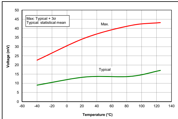
FIGURE 36-56: LPBOR Reset Hysteresis.
