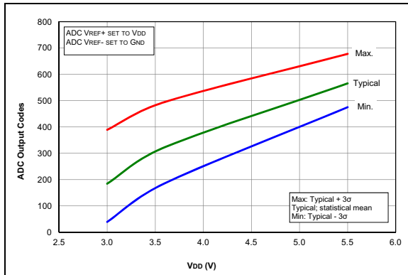
FIGURE 36-73: Temp. Indicator Initial Offset, High Range, Temp. = 20^\circ\text{C} , PIC16F1614/8 Only.
