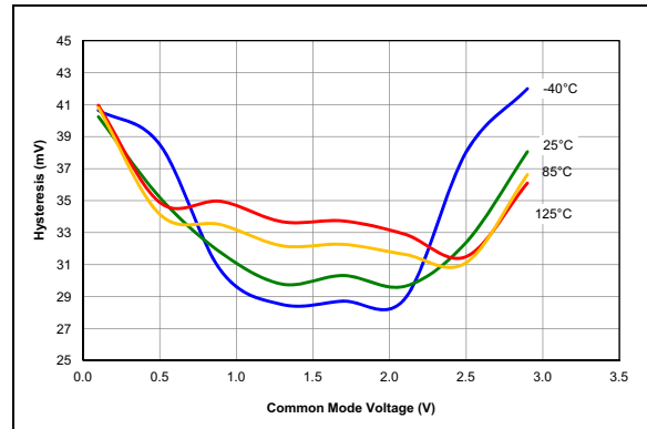
FIGURE 36-82: Comparator Hysteresis, NP Mode ( CxSP = 1 ), V_{DD} = 3.0V , Typical Measured Values.
