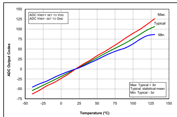
FIGURE 36-78: Temp. Indicator Slope Normalized to 20^\circ\text{C} , Low Range, V_{DD} = 3.0V , PIC16F1614/8 Only.
