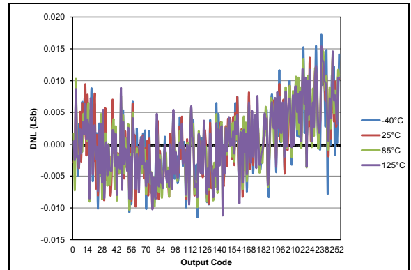
FIGURE 36-94: Typical DAC INL Error, V_{DD} = 5.0V , V_{REF} = \text{External } 5V , PIC16F1614/8 Only.
