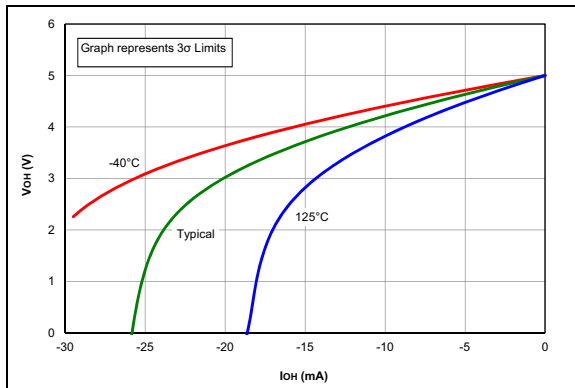
FIGURE 36-37: V_{OH} vs. I_{OH} Over Temperature, V_{DD} = 5.0V , PIC16F1614/8 Only.
