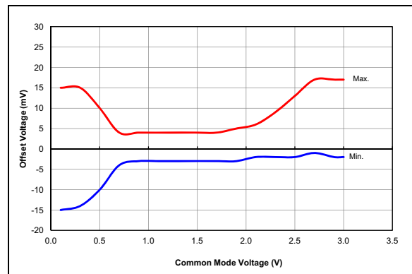
FIGURE 36-83: Comparator Offset, NP Mode ( CxSP = 1 ), V_{DD} = 3.0V , Typical Measured Values at 25^\circ\text{C} .
