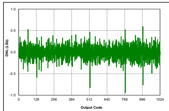
FIGURE 36-66: ADC 10-bit Mode, Single-Ended DNL, V_{DD} = 3.0V , T_{AD} = 4\text{ }\mu\text{s} , 25^\circ\text{C} .
