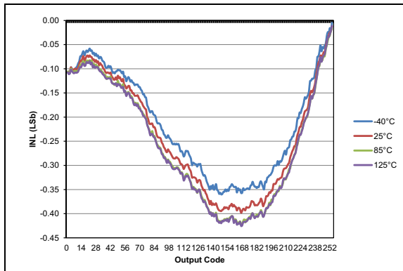
FIGURE 36-93: Typical DAC INL Error, V_{DD} = 3.0V , V_{REF} = \text{External } 3V .
