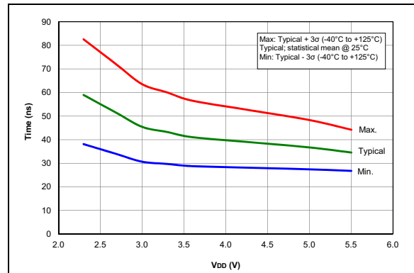
FIGURE 36-89: Comparator Response Time Over Voltage, NP Mode ( CxSP = 1 ), Typical Measured Values, PIC16F1614/8 Only.
