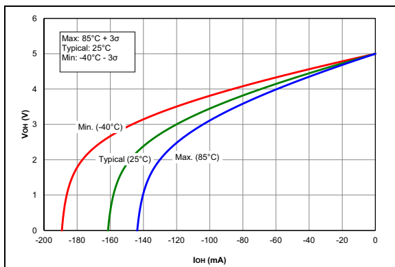
FIGURE 36-39: V_{OH} vs. I_{OH} Over Temperature for High Drive Pins, V_{DD} = 5.0V , PIC16F1614/8 Only.
