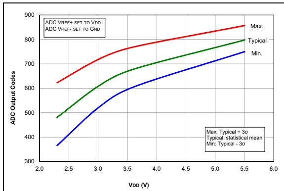
FIGURE 36-74: Temp. Indicator Initial Offset, Low Range, Temp. = 20^\circ\text{C} , PIC16F1614/8 Only.
