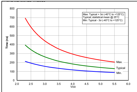
FIGURE 36-91: Comparator Output Filter Delay Time Over Temp., NP Mode ( C_{xSP} = 1 ), Typical Measured Values, PIC16F1614/8 Only.
