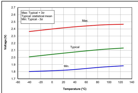
FIGURE 36-55: LPBOR Reset Voltage.
