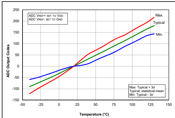
FIGURE 36-79: Temp. Indicator Slope Normalized to 20^\circ\text{C} , Low Range, V_{DD} = 1.8V , PIC16LF1614/8 Only.
