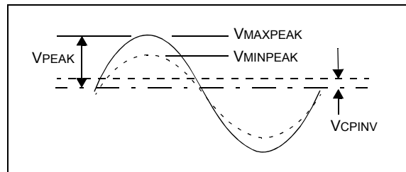
FIGURE 21-1: EXTERNAL VOLTAGE
