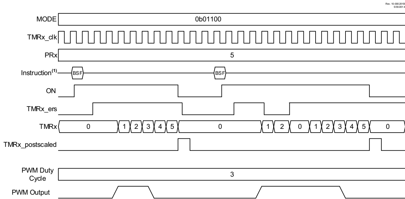
FIGURE 29-10: EDGE-TRIGGERED HARDWARE LIMIT ONE-SHOT MODE TIMING DIAGRAM (MODE = 01100)
