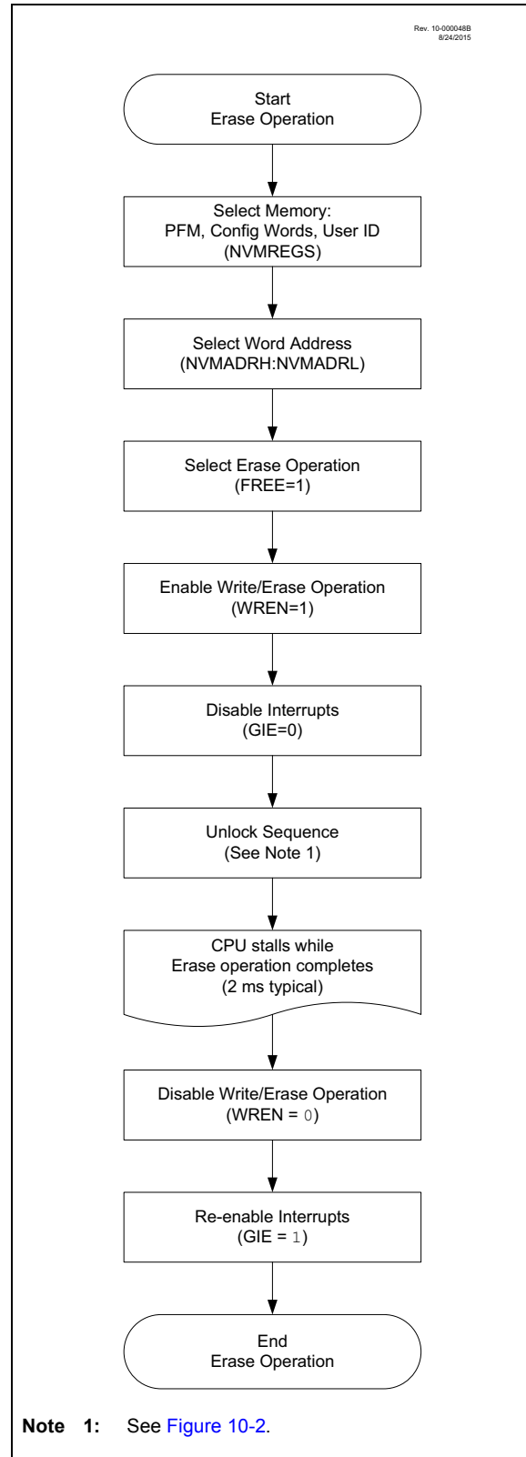
FIGURE 10-3: NVM ERASE FLOWCHART
