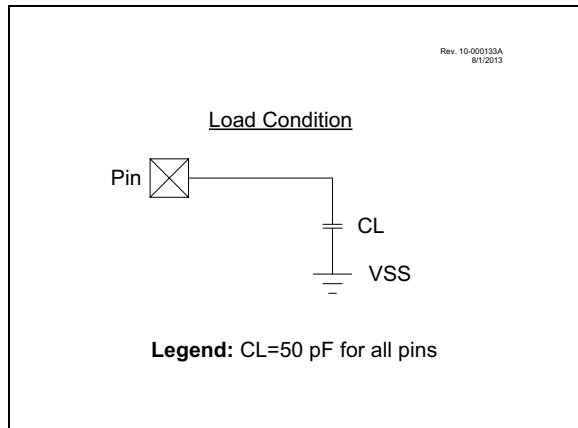
FIGURE 37-4: LOAD CONDITIONS
