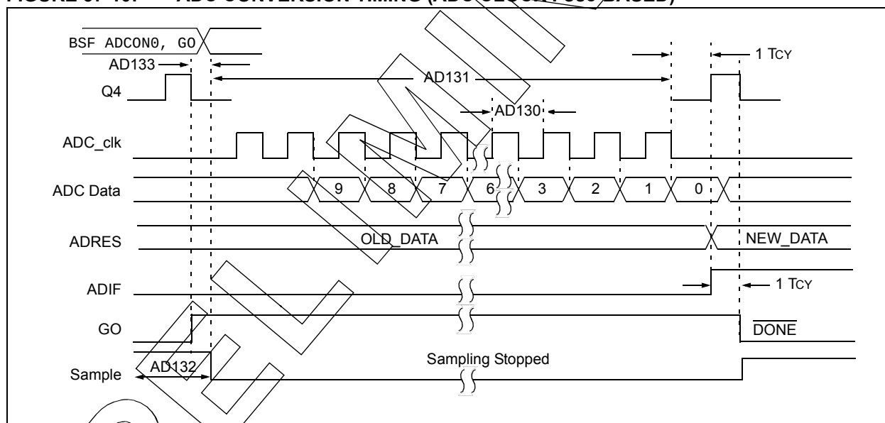
FIGURE 37-10: ADC CONVERSION TIMING (ADC CLOCK Fosc-BASED)
