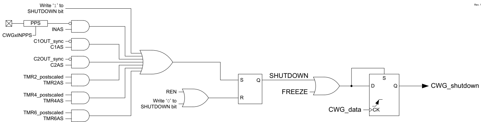
FIGURE 20-12: CWG SHUTDOWN BLOCK DIAGRAM
